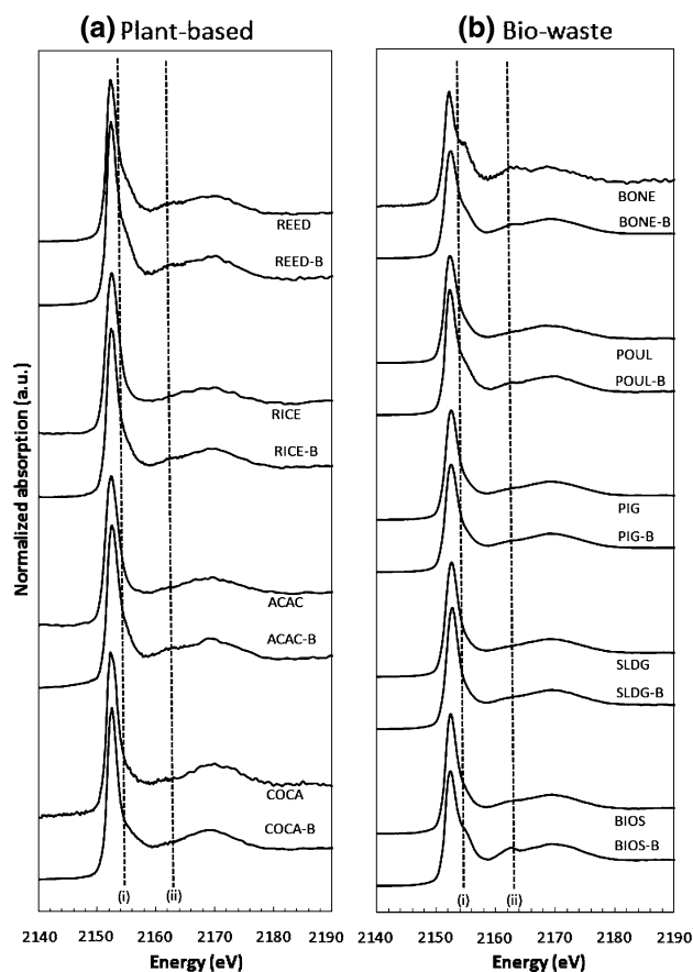
Fig. 1 Stacked normalised P K-edge XANES spectra of the biomass feedstocks and their derived biochars (-B): a plant-based and b bio-waste materials. Sample identification is explained in the “Materials and methods” section
