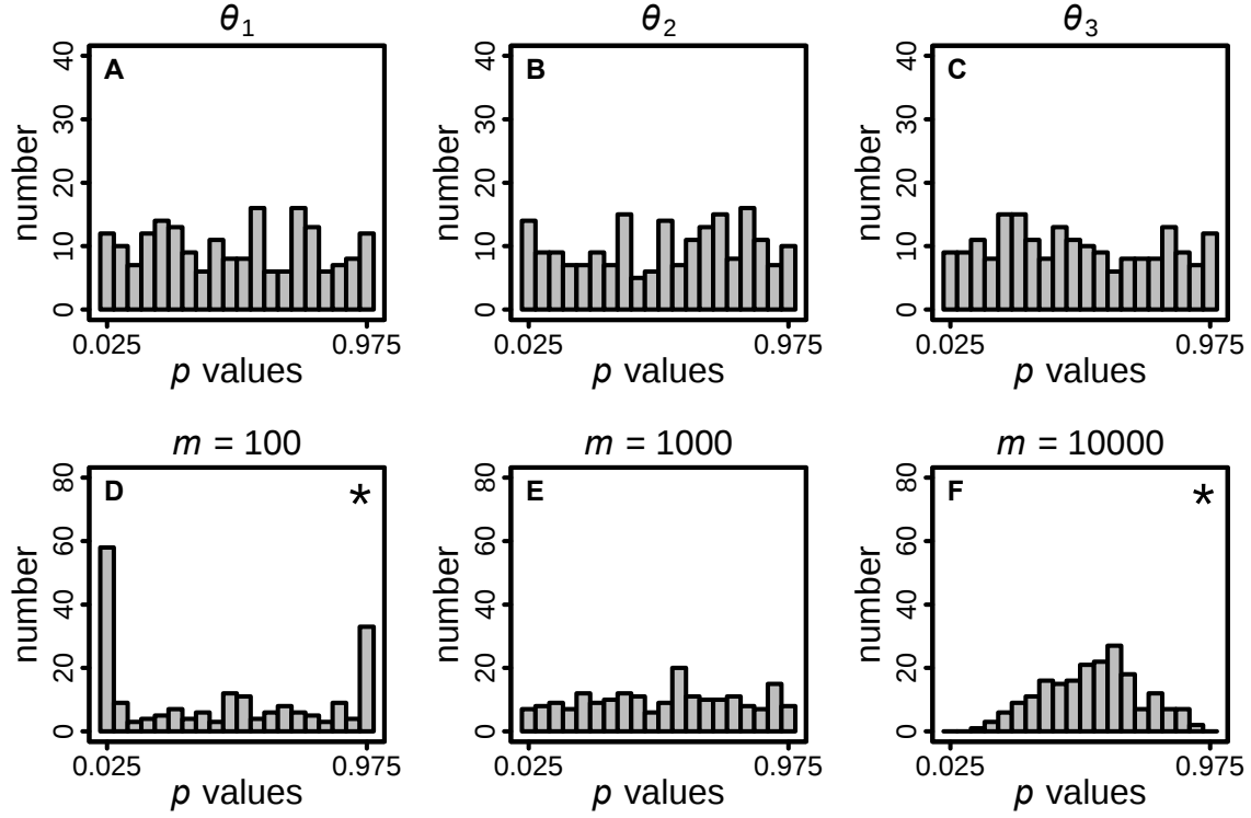
Figure 2. Coverage for the quadratic example. A - C: ‘Error-calibrated ABC’. D – F: ‘Rejection ABC’ for parameter \theta_3 at different acceptance rates m . Asterisks mark significant departures from uniformity (Kolmogorov-Smirnov, p < 0.01 ).
