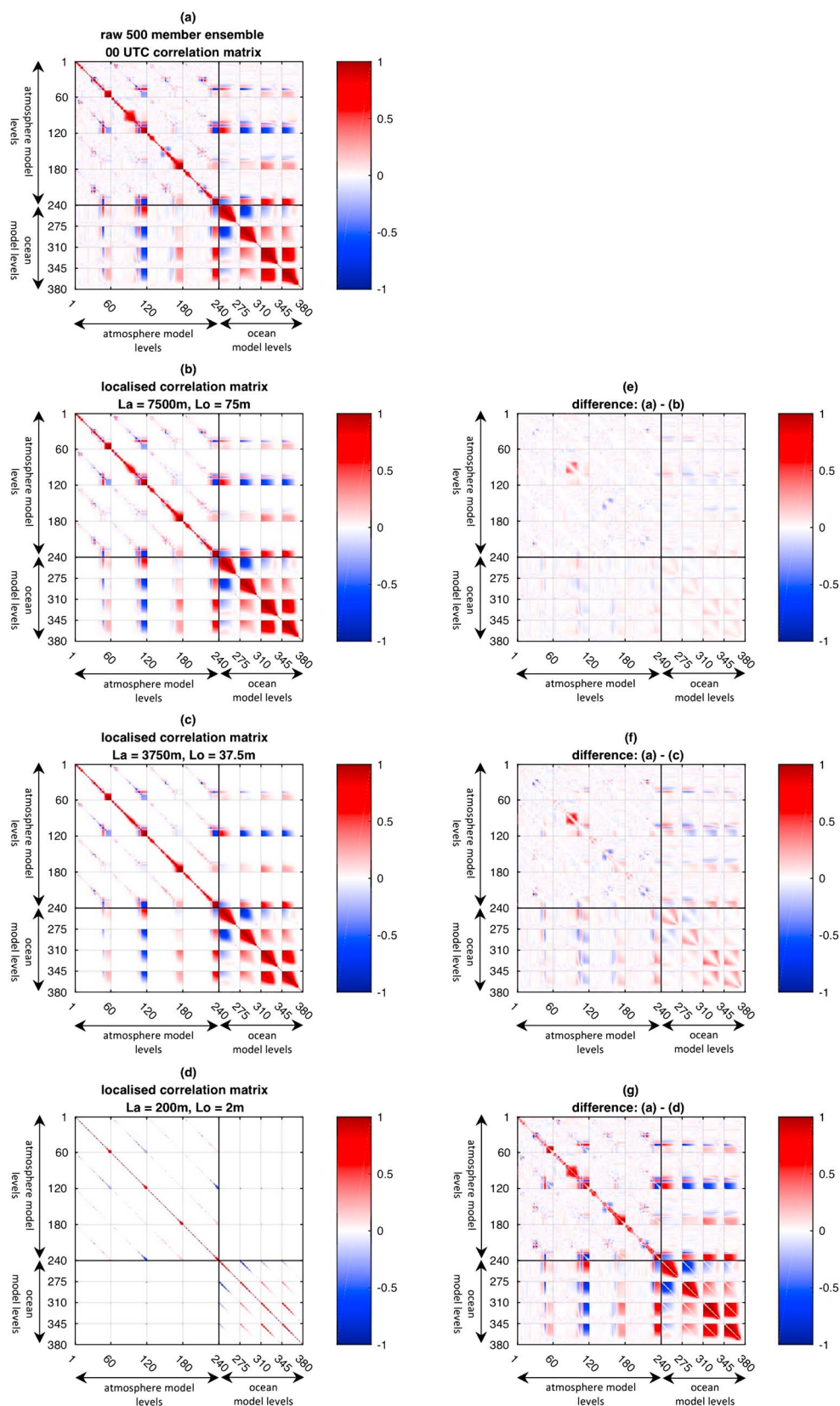
Figure 2. Comparison of the structure of (a) the original ensemble error correlation matrix and the localized error correlation matrix for length scales: (b) L_a = 7,500\text{ m} , L_o = 75\text{ m} ; (c) L_a = 3,750\text{ m} , L_o = 37.5\text{ m} ; and (d) L_a = 200\text{ m} , L_o = 2\text{ m} . (e–g) Show the difference between Figures 2a and 2b–2d. Model levels are as in Figure 1.
