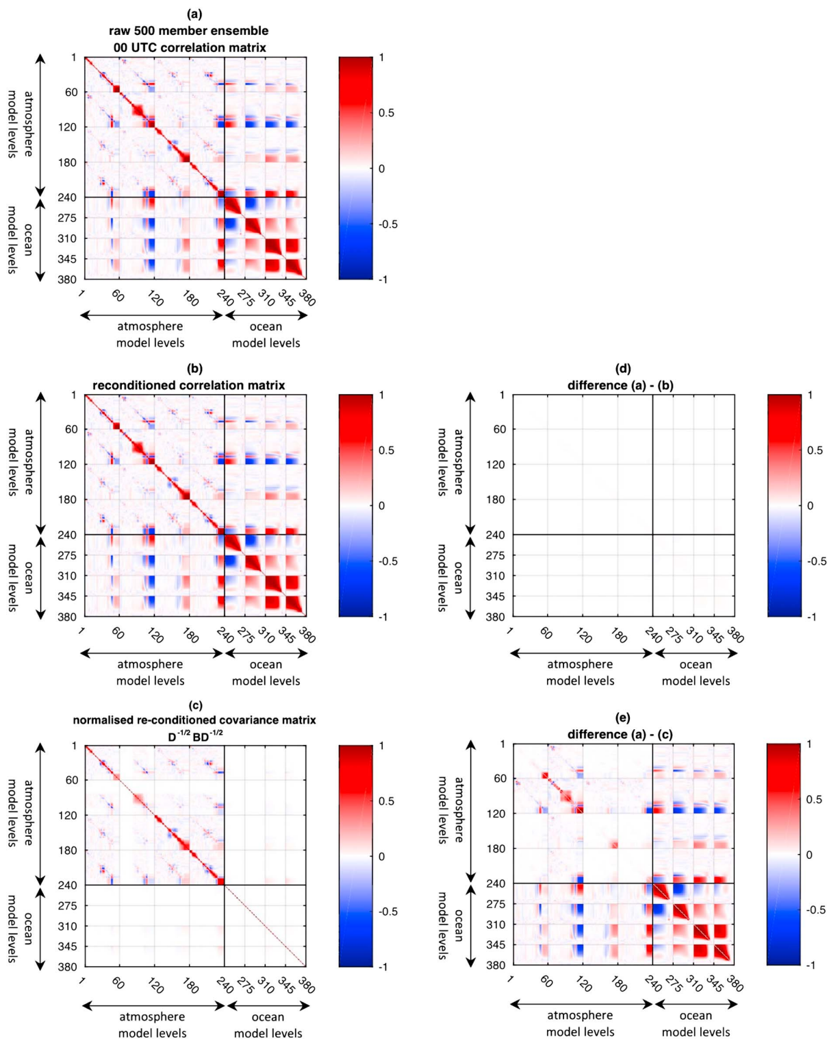
Figure 1. Comparison of the structure of (a) the original ensemble error correlation matrix, (b) the reconditioned error correlation matrix, and (c) the normalized reconditioned error covariance matrix when \kappa_{tol} = 10^4 . (d and e) Show the difference between Figures 1a and 1b, 1c. Model levels 1–240 correspond to atmosphere temperature, specific humidity, and zonal and meridional wind on 60 levels; model levels 241–380 correspond to ocean temperature, salinity, and zonal and meridional current on 35 levels.
