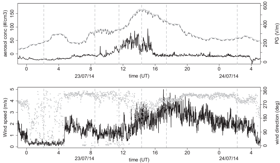
Fig. 5. (a) Aerosol number concentration (solid light grey = total concentration for all particles from 0.3–10 μm, dashed dark grey = concentration of particles < 1 μm), measured by a TSI3330 OPC. The black line shows measurements of Potential Gradient (PG) measured by a JCI 131F electric field mill. (b) 2 m wind speed (black solid line) and wind direction (grey points), all measured at Alqueva, Portugal on 23rd and 24th July 2014. Dashed grey lines denote the times of balloon ascents. Aerosol measurements are 5 minute averages, PG 1 minute averages and wind data 1 minute average.
