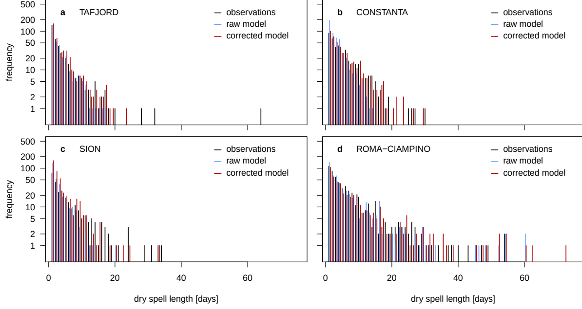
Figure 2: Unrealistic dry spell lengths | Distribution of dry spell lengths (wet-day threshold 0.1 mm) at a , Tafjord (Norway; 7.41° W, 62.23°N, winter), b , Constanta (Romania; 28.63° E, 44.22°N, winter), c , Sion (Switzerland, 7.33° E, 46.22°N, winter) and d , Rome (Italy, 12.58° E, 41.78°N, summer) of MPI-ESM-LR downscaled with CLM to a horizontal resolution of 0.44°, 1971-2000. Black: observations (ECA-D 90 ), blue: raw climate model, red: corrected climate model. Long dry spells are typically underrepresented even after a seasonal wet day correction ( a ), although in some cases the correction may improve the overall distribution ( b ). Often, artefacts are introduced for short ( c ) and long ( d ) spells.
