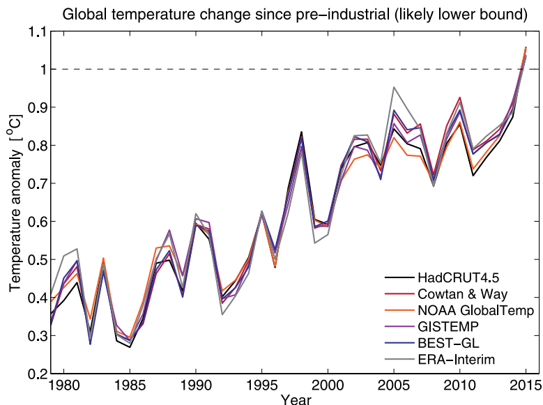
FIG. 5. Global mean temperature relative to preindustrial in six datasets, using the likely lower bound ( 0.60^{\circ}\text{C} ) for warming from preindustrial to 1986–2005. The change in the ERA-Interim reanalysis (Dee et al. 2011) relative to 1986–2005 is included with the five global temperature datasets discussed. The 1996–2015 period is 0.16^{\circ}\text{--}0.19^{\circ}\text{C} warmer than 1986–2005.
