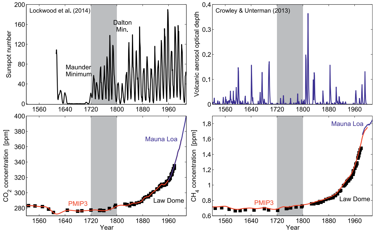
FIG. 1. Historical natural forcings and greenhouse gas variations. (top left) Annual sunspot number since 1612, with the Maunder Minimum and Dalton Minimum indicated (Lockwood et al. 2014). (top right) Estimated global volcanic aerosol optical depth (Crowley and Unterman 2013). (bottom) The Law Dome greenhouse gas data (MacFarling Meure et al. 2006; black) for (left) carbon dioxide and (right) methane, along with the annual means from Mauna Loa (Keeling et al. 2001; blue) and PMIP3 assumed values (Schmidt et al. 2012; red). Note there is a 16 ppb offset applied to the smoothed Law Dome methane concentrations to produce a global mean as used by PMIP3 to account for the interhemispheric gradient. The 1720–1800 period is denoted by the gray shaded region in all panels.
