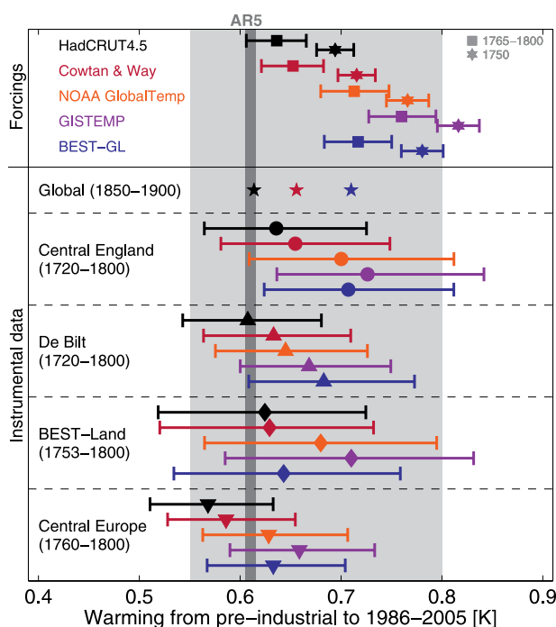
FIG. 4. Summarizing the evidence for annual-mean global temperature change from preindustrial until 1986–2005 using each dataset. The horizontal bars represent the 5%–95% uncertainty ranges for the different sources of evidence. Results for the radiative forcing approach are shown averaged over 1765–1800 and for 1750. The top row in the instrumental observations section shows the observed change since 1850–1900 (where available). For the instrumental data the longest time series during the preindustrial period are used: CET and De Bilt (1720–1800), BEST-Land (1753–1800), and central Europe (1760–1800). The light gray shading shows the assessed likely range and the dark gray line indicates the IPCC AR5 assessment (0.61°C; Kirtman et al. 2013).
