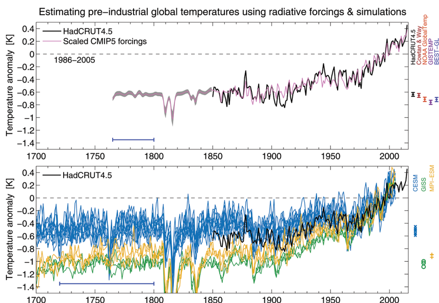
FIG. 2. (top) Estimating global preindustrial temperature using scaled radiative forcings (pink), using HadCRUT4 (black) as the reference. The gray shading represents the uncertainty in the regression. Estimated global temperature anomalies for 1765–1800 are given for all five global temperature datasets (right-hand side, as labeled). (bottom) Simulated global temperature anomalies in the LMEs and estimates for the change since 1720–1800 for the range of ensemble members of CESM (blue), GISS (green), and MPI-ESM (orange). In both panels the blue horizontal bars indicate the period used for averaging. Temperature anomalies are presented relative to the mean of the reference period 1986–2005 (dashed black line).
