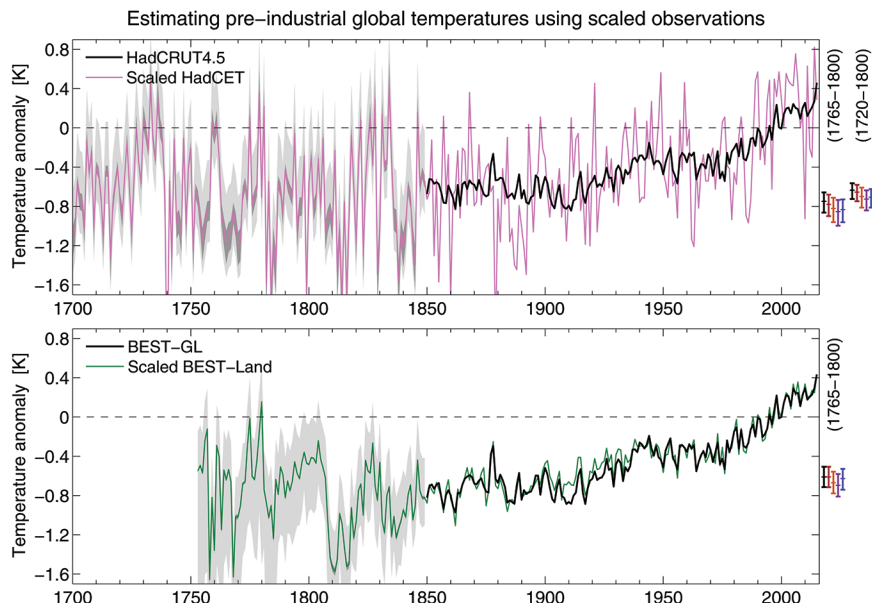
FIG. 3. Estimating global preindustrial temperature using scaled annual-mean observations for (top) CET scaled to HadCRUT4 and (bottom) BEST-Land scaled to BEST-GL, relative to 1986–2005 (dashed black). The dark gray shading (hardly visible) represents the uncertainty in the regressions and the light gray shading the uncertainty in the observations. The sets of five error bars on the right-hand side use the different global temperature datasets, with the same ordering as in the top panel of Fig. 2, for the two different averaging periods as labeled. Note the vertical scale is different from Fig. 2.
