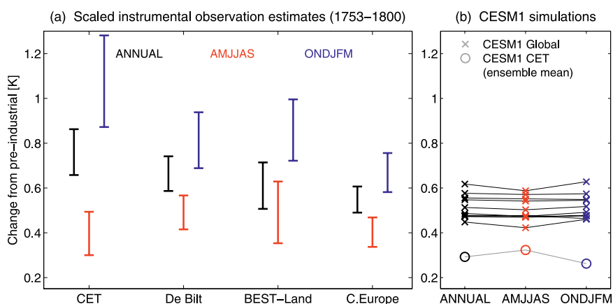
FIG. A1. Seasonal differences in warming rates. (a) Derived scaled warming from 1753–1800 to 1986–2005 (using approach 3) for annual means (black) and for the extended seasons (Apr to Sep—AMJJAS, red; and Oct to Mar—ONDJFM, blue) for the different regional time series, all using annual-mean HadCRUT4 as the reference dataset. (b) Seasonal warming derived from the CESM1 LME simulations for the global mean (crosses, with black lines linking the same ensemble members in each season) and for the ensemble mean of simulated CET (circles).
