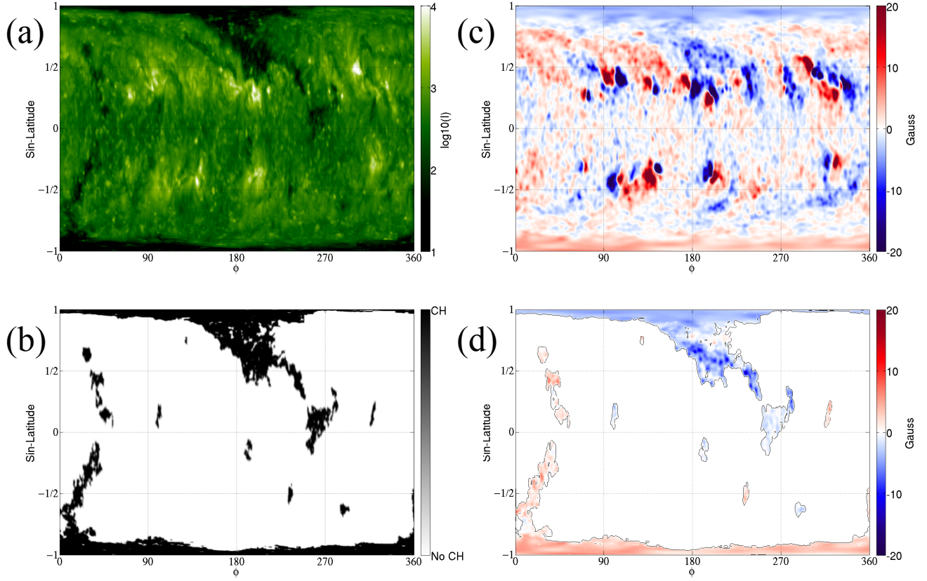
Fig. 3.— (a) Diachronic EUV map for CR2098 (6/16-7/13/2010), constructed predominantly from AIA 193Å images, plotted as sine(latitude) vs. longitude (b) Corresponding CH detections for (a), plotted in the same format. (c) B_r at the photosphere derived from the LOS field, for data from the NSO VSM for this Carrington rotation. (d) The magnetic field in the CH, obtained by overlaying (b) with (c).
