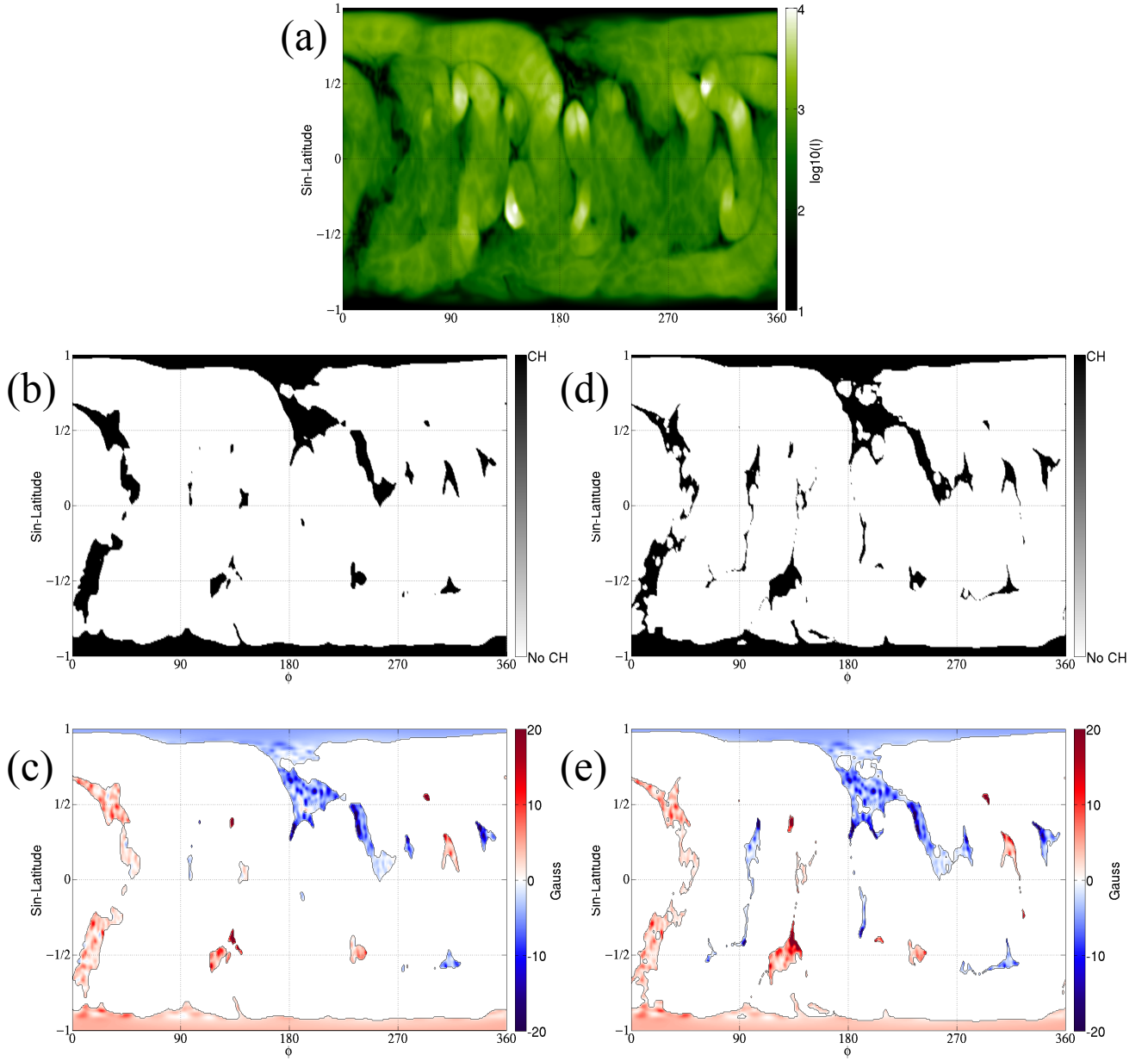
Fig. 4.— (a) Simulated AIA 193Å map from the thermodynamic MHD model using the NSO VSM CR2098 map for the boundary condition. This map is used to test the CH detection method. (b) The CHs (black regions) identified when the CH detection method is applied to the simulated data. (c) The magnetic field in the CH, obtained by overlaying (b) with the NSO VSM map (as was done in Figure 3). (d) The true open field regions for the model. (e) The true open magnetic field in the model.
