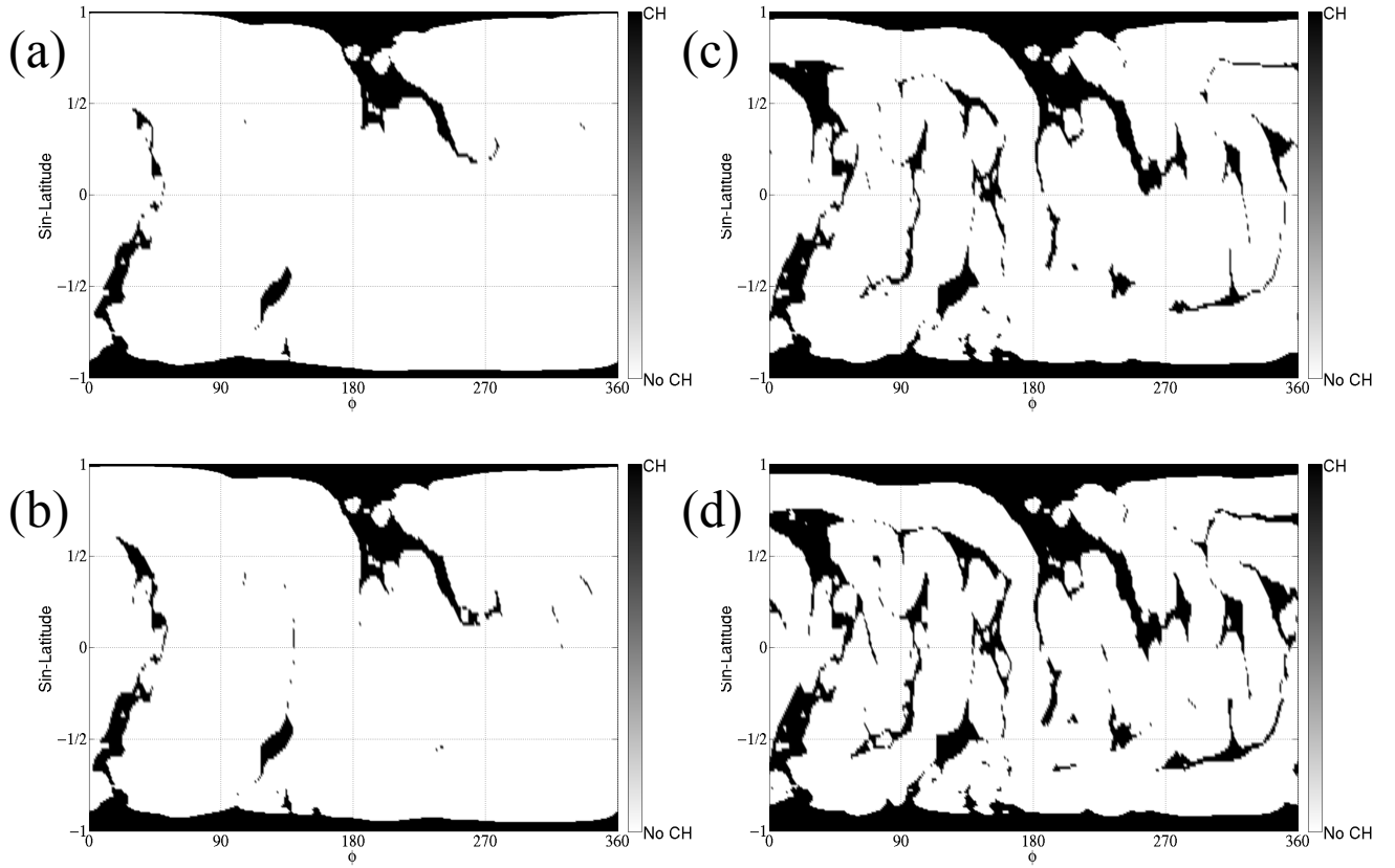
Fig. 2.— Open field regions (black) for four PFSS models using the NSO VSM CR2098 map for the boundary condition. (a) R_{SS} = 2.5R_S . (b) R_{SS} = 2.0R_S . (c) R_{SS} = 1.4R_S . (d) R_{SS} = 1.3R_S .
