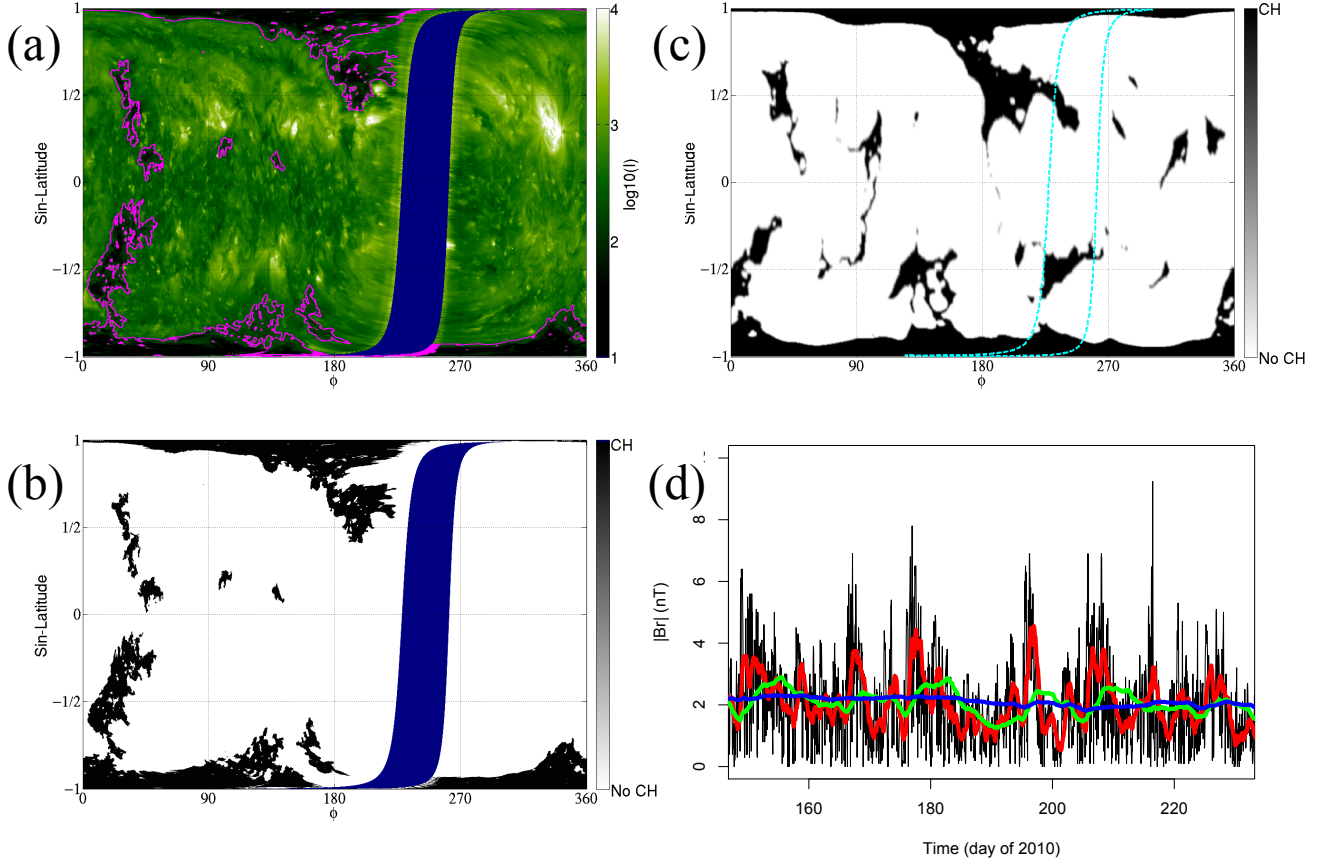
Fig. 1.— (a) Synchronic EUV map for July 8, 2010 at 18:00, compiled from STEREO A & B EUVI 195\text{\AA} and SDO AIA 193\text{\AA} images. The magenta lines show the coronal hole detections. The sector near 270^\circ , indicated by the blue swath, was not observed. (b) The detected coronal holes (black regions) from (a). (c) Open field regions (black) from a thermodynamic MHD model with boundary derived from an ADAPT map. The unobserved region is indicated with cyan dashed lines. (d) OMNI in situ measurements of B_r for 80 days surrounding the time period of interest. A 1-hour running average of |B_r| (black line), 1-day running average (red), 7-day (green) and Carrington rotation average (blue) are shown.
