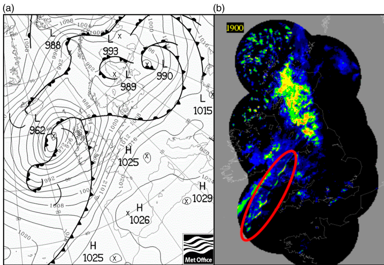
FIG. 3. (a) Met Office surface analysis at 0000 UTC 25 Nov 2009 and (b) Met Office radar-derived precipitation rates at 1900 UTC 24 Nov 2009. The positions of the NCFR are highlighted in the radar image.
