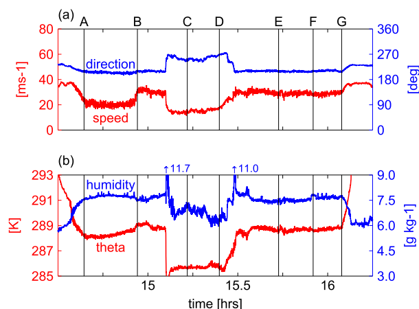
FIG. 4. Time series of observed (a) wind speed and direction, and (b) potential temperature and specific humidity. The aircraft altitude was 40 m during leg AB and 300 m during circuit BG, with the ascent beginning 1 min before point B. The locations of points A–G are indicated in Fig. 1.
