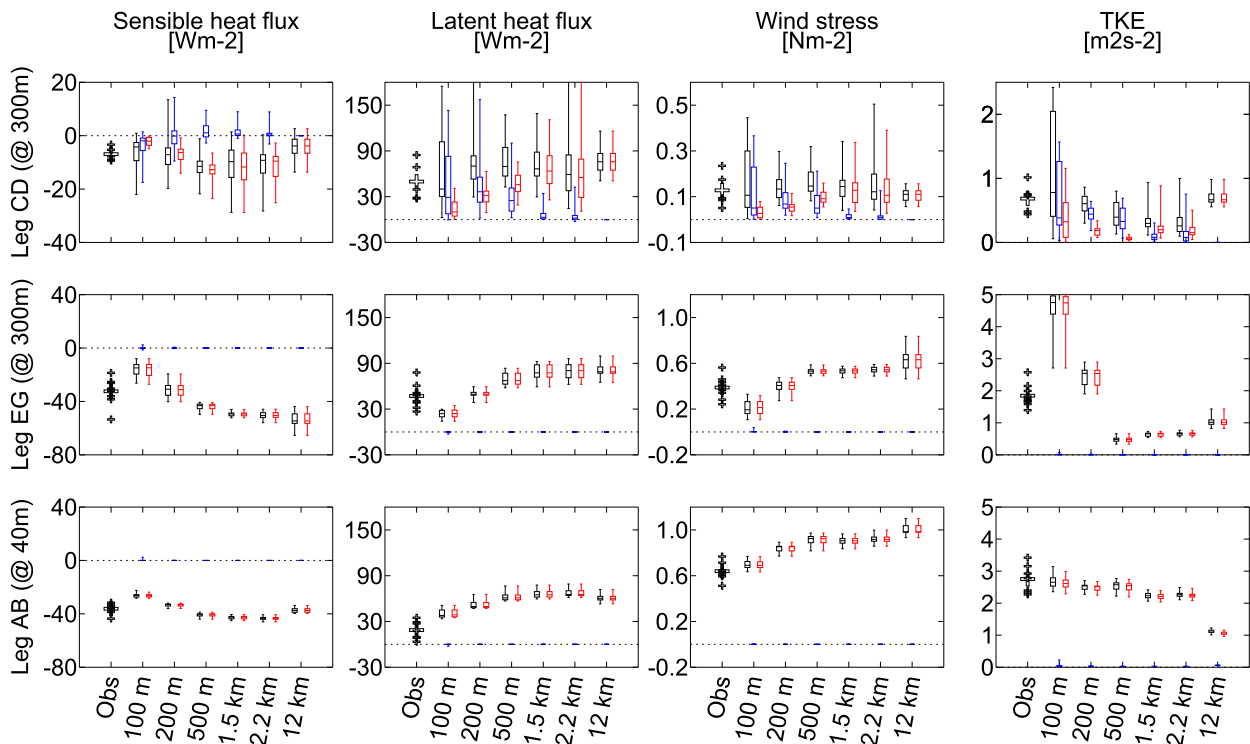
FIG. 10. Summary of observed (crosses) and simulated (box and whisker) turbulent fluxes along (top) the cold side of front at 300 m, (middle) the warm side of front at 300 m, and (bottom) the warm side of front at 40 m. For the observations the large cross shows the leg-average value and the small crosses show the values of the individual 2-min runs. For the model simulations, the three bars indicate the median, interquartile range, and full range of leg-average values from the sample of circuits for the parameterized (red), resolved (blue), and total (parameterized plus resolved; black) fluxes.
