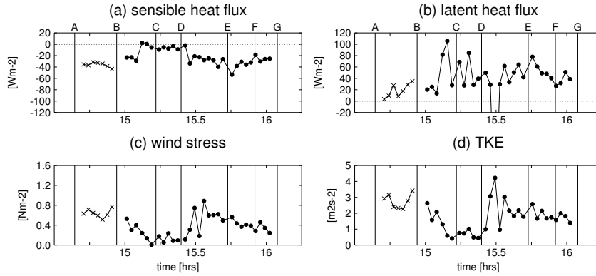
Figure 9: Timeseries of (a) sensible heat flux, (b) latent heat flux, (c) wind stress and (d) turbulent kinetic energy. Each dot (cross) represents the eddy covariances calculated from 32 Hz data over straight and level two-minute legs at 300 m (40 m) altitude, as described in the text.
