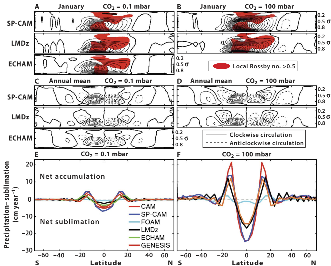
Fig. 9. More Snowball Earth intermodel comparisons (81). See Fig. 8 caption for the prescribed conditions. January mean mass Eulerian stream function for models SP-CAM, LMDz, and ECHAM at (A) CO 2 = 0.1 mbar and (B) CO 2 = 100 mbar. \sigma is air pressure as a fraction of the surface air pressure. Clockwise atmospheric circulation is depicted by thin solid lines, counterclockwise circulation is depicted by thin dashed lines, and the zero stream function is depicted by thick solid lines. Contour interval is 50 \times 10^9 \text{ kg s}^{-1} . Maximum mass stream functions in January increase by a factor of \sim 1.5 between 0.1 and 100 mbar of CO 2 . ECHAM is unstable at CO 2 = 100 mbar. Note the ascending flow in January between 10°S and 30°S and the descending flow between 10°S and 20°N. Red shade indicates regions where the local Rossby number is greater than 0.5, meaning that inertial forces dominate over Coriolis forces. (C and D) Same as (A) and (B) but depict the annual mean mass Eulerian stream function. Contour interval is 20 \times 10^9 \text{ kg s}^{-1} . Note that air descends in the inner tropics in the annual mean and ascends in the subtropics. This governs the surface hydrologic balance (E and F). Annual and zonal mean precipitation minus sublimation with (E) CO 2 = 0.1 mbar and (F) CO 2 = 100 mbar. Note the net sublimation in the inner tropics and the net accumulation in the near subtropics, opposite to the present climate. The hydrologic cycle amplifies by nearly a factor of 10 between 0.1 and 100 mbar of CO 2 but is muted in FOAM due to cold surface temperatures (Fig. 8, A and B). LMDz exhibits grid-scale noise in (F).
