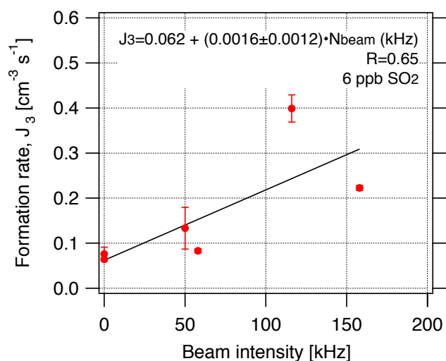
Fig. 8. Particle formation rate, J_3 , vs. beam intensity, at 6 ppb [\text{SO}_2] . The measurements are listed in Table 1 (“negative” formation rates – corresponding to aerosol particle sinks – are not plotted).
