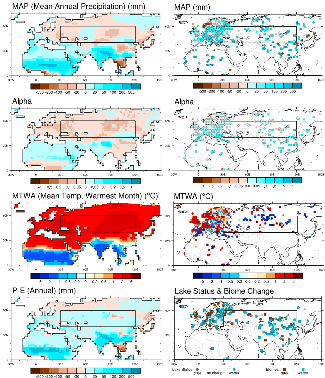
Figure 1. (left column) Long-term mean differences ( midHolocene minus \pi iControl) of mean annual precipitation (MAP), the Cramer-Prentice index of soil moisture availability (Alpha), mean temperature of the warmest month (MTWA), and precipitation minus evaporation ( P - E ), calculated as in Harrison et al. [2014], and (right column) paleoclimatic reconstructions of mid-Holocene minus present values of MAP, Alpha, and MTWA [ Bartlein et al. , 2011], along with lake status and biome change inferred differences in moisture (see data sources in the supporting information). The region of interest here (40° to 60°N and 30° to 120°E) is indicated by the gray box in each panel.
