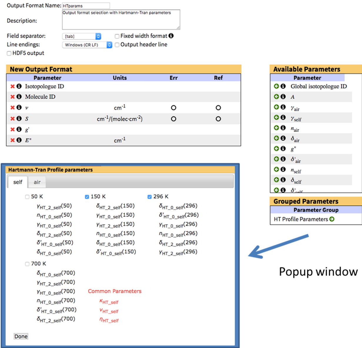
Fig. 30. Groups of related parameters such as those relating to the HT profile in different temperature regions are selected from a separate set of overlay panels in the HITRANonline interface. When one or more temperature groups are chosen, the three "Common parameters" are also automatically selected. Conversely, these common parameters are removed from the selection when no temperature group is chosen for this profile. Different broadening species are presented on separate panels, and may be selected from the labeled tabs at the top of the overlay.
