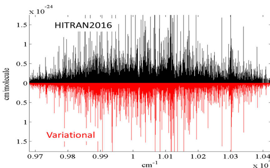
Fig. 15. Comparison of unassigned experimental line list of ^{12}\text{CH}_4 in the Tetracontad range (Béguier et al. [197]) included in HITRAN2016 (upper panels in black) with variational calculations, Rey et al. [205] based on ab initio dipole moment [202], and potential energy [203,204] surfaces using the line list included in the TheoReTS database [205] (lower panel upside down in red).
