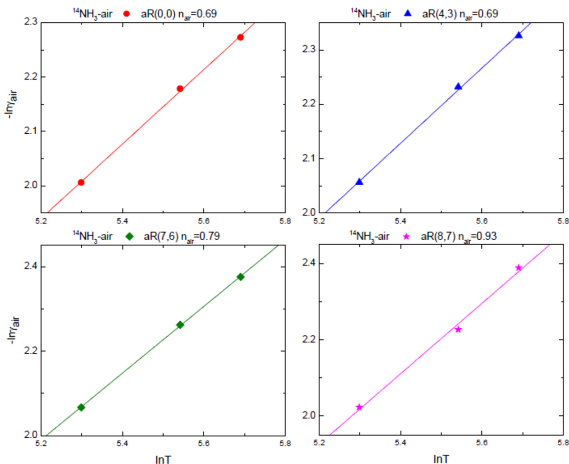
Fig. 19. Air-broadening line widths of \text{NH}_3 with different temperatures for \text{aR}(0,0) , \text{aR}(4,3) , \text{aR}(7,6) and \text{aR}(8,7) transitions. The temperature-dependence exponent n_{\text{air}} is determined from the slope of the least-squares fits of -\ln\gamma_{\text{air}}^0(T) vs. \ln T .
