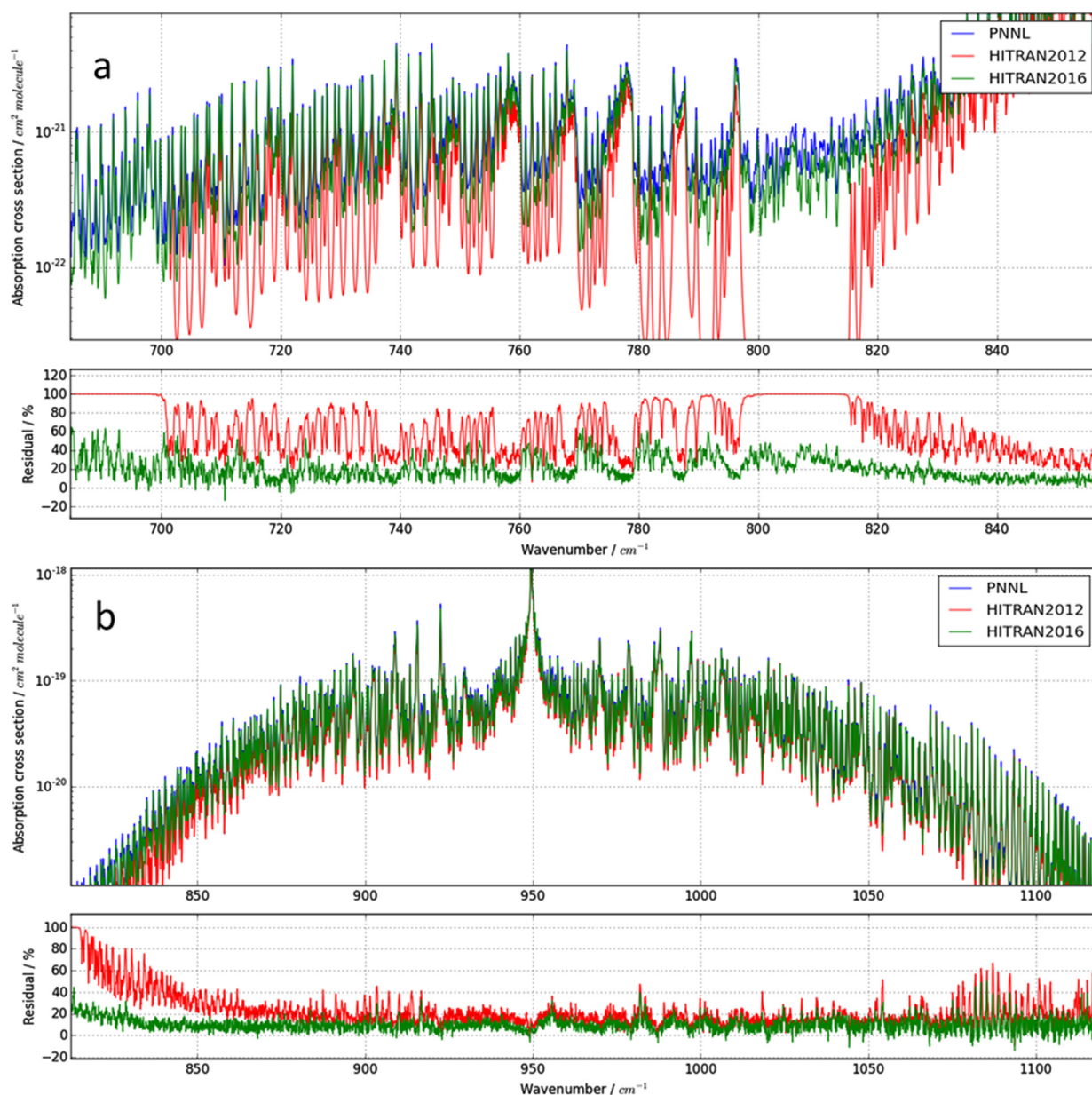
Fig. 25. HITRAN2016 vs HITRAN2012 when simulating PNNL experimental data in the a) 700–850 cm -1 , b) in the 850–1100 cm -1 regions of ethylene spectra (1 atm., 296 K).
