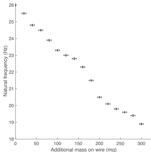
FIG. 4. Response of the 0.5 mm vibrating wire's natural frequency to an incremental mass increase. A linear fit indicates a sensitivity of -0.02 \text{ Hz mg}^{-1} with a standard error of 0.27 Hz and an R^2 of 0.99. Vertical error bars represent the frequency measurement precision of \pm 0.05 Hz and horizontal error bars represent the mass measurement precision of \pm 5 mg.
