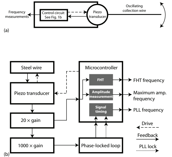
FIG. 1. (a) Sketch of the oscillating microbalance collector. (b) Block diagram to illustrate the main components and signal flow. Dashed lines show optional drive provided to the piezo transducer, dotted lines show the PLL 'lock' state signal, and solid lines show the signal received from the wire vibration. White boxes indicate hardware and grey boxes indicate software. Signal flow and component definitions are described in the text.
