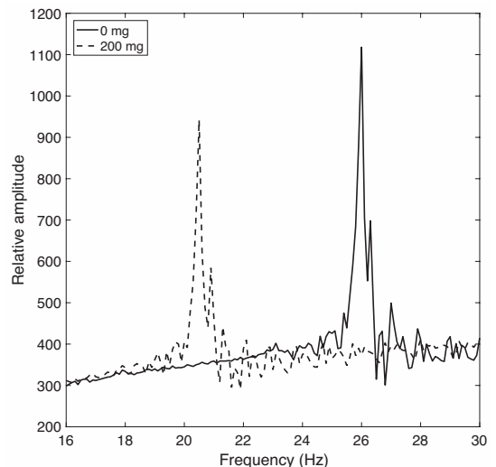
FIG. 2. Relative amplitude frequency response of a 120 mm long, 0.5 mm diameter steel wire after being driven for short pulse intervals ( \sim 1 s) at 0.1 Hz steps over a range of frequencies. The solid line is for an unladen wire and the dashed line is for the same wire loaded evenly with an additional 200 mg of material.
