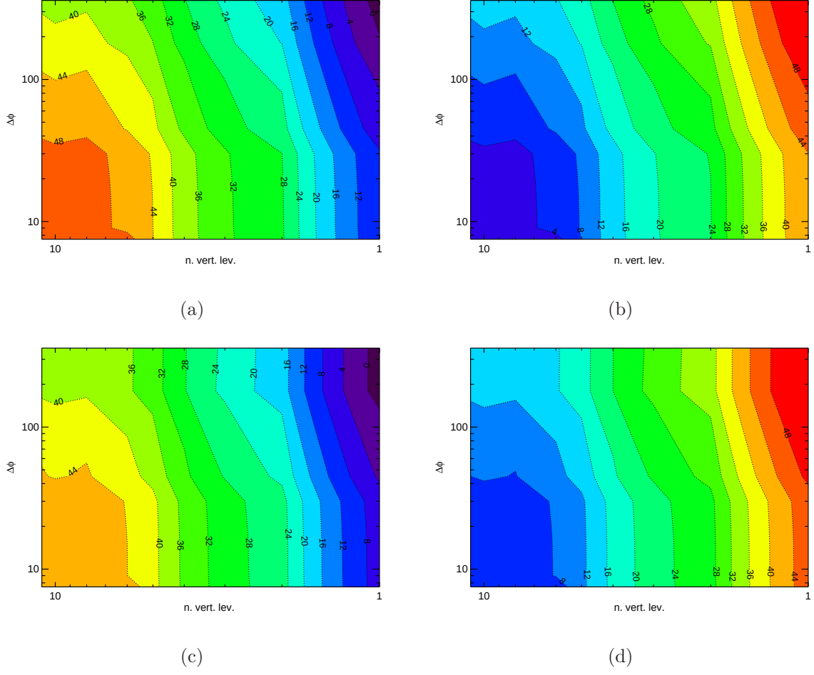
FIG. 6. Estimates of \overline{\langle \dot{S}_{mat}^{ind} \rangle_v}^\tau (a), and \Delta \left[ \dot{S}_{mat}^{ind} \right]_v^\tau (b) for \tau = 1 day, and of \overline{\langle \dot{S}_{mat}^{ind} \rangle_v}^\tau (c), and \Delta \left[ \dot{S}_{mat}^{ind} \right]_v^\tau (d) for \tau = 1 year. The spatial averaging considered here is given by areal averages along horizontal surfaces and vertical averages along columns. The x -axis reports the numbers of vertical levels involved in the averaging, the y -axis describes the longitudinal extent \Delta\phi of the coarse grained grid boxes. Details are given in the text.
