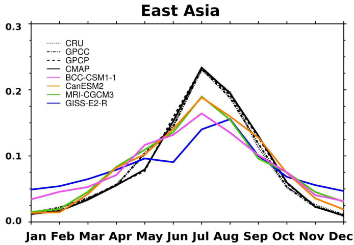
Fig. 13 Precipitation frequencies p_m = r_m/R for observation datasets CRU, GPCC, GPCP, CMAP and four models (BCC-CSM1-1, CanESM2, MRI-CGCM3 and GISS-E2-R) over East Asia.
