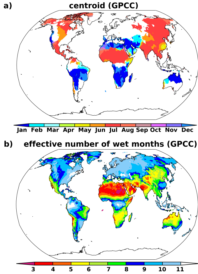
Fig. 15 Centroid (a) and effective number of wet months (b) of the monthly precipitation sequence p_m for the GPCC dataset. In (a) numbers denotes the months of the year around which p_m is centered and in (b) the length in months. The centroid is not shown for regions with D \geq 0.2 – corresponding approximately to n' greater than 11.
