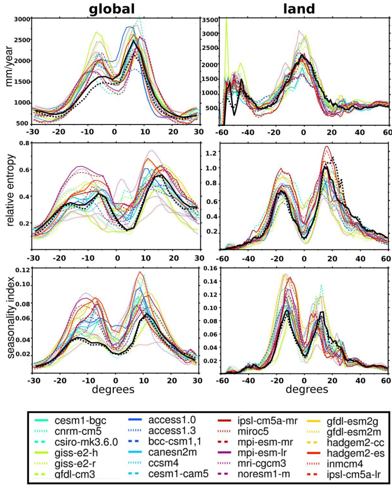
Fig. 7 Left column: zonal means of precipitation, relative entropy and dimensionless seasonality index over the whole globe (GPCP and CMAP observation dataset are denoted with black continuous and dashed line respectively) for the period 1979-2008. Right column: as before but over land only (GPCP and CRU are denoted with black continuous and dashed line respectively).
