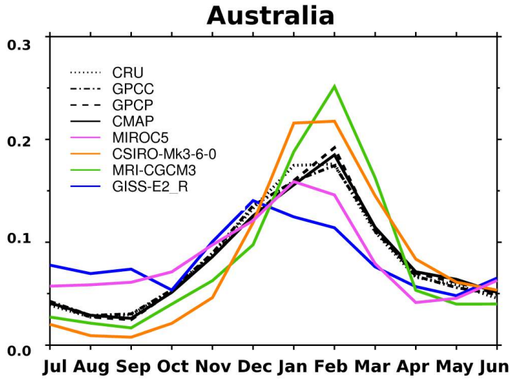
Fig. 10 Precipitation fractions p_m = r_m/R for observation datasets CRU, GPCC, GPCP, CMAP and four models (CSIRO-Mk3-6-0, MRI-CGCM3, MIROC5 and GISS-E2-R) over Australia.
