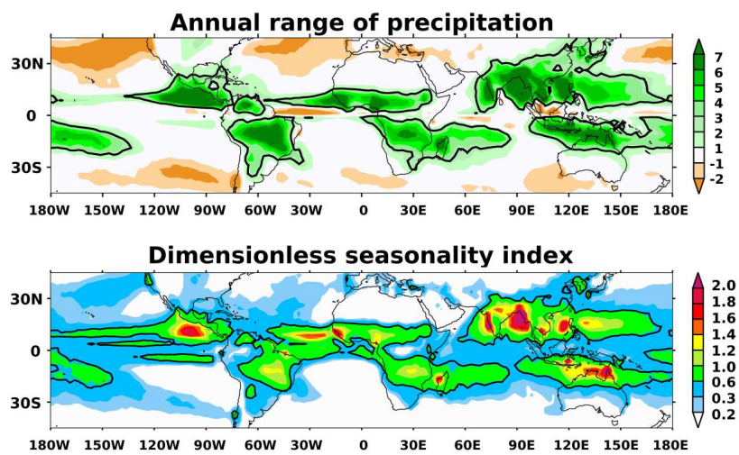
Fig. 5 Annual range of precipitation (mm/day) and DSI ( \times 10 ) for the CMAP climatology. The global monsoon domain ( black thick line ) is defined by the annual range equal to 2.5 mm/day and DSI equal to 0.05.
