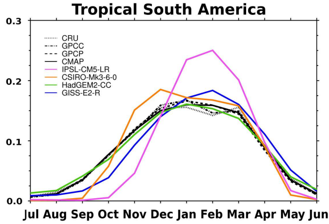
Fig. 9 Precipitation frequencies p_m = r_m/R for observation datasets CRU, GPCC, GPCP, CMAP and four models (CSIRO-Mk3-6-0, IPSL-CM5-LR, HadGEM2-CC and GISS-E2-R) over tropical Latin America.
