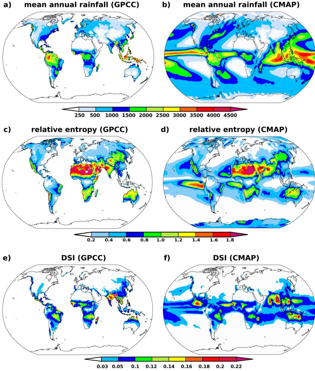
Fig. 1 (a, b) Mean annual rainfall \bar{R} (mm yr -1 ), (c, d) relative entropy \bar{D} and (e, f) dimensionless seasonality index \bar{S} for the GPCC land dataset (left column) and CMAP dataset (right column).
