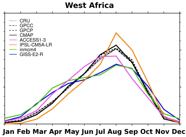
Fig. 12 Precipitation fractions for observation datasets CRU, GPCC, GPCP, CMAP and four models (IPSL-CM5A-LR, Inmcm4, ACCESS1-3 and GISS-E2-R) over western Africa
