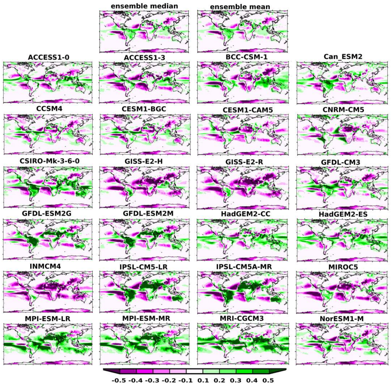
Fig. 8 As in Fig. 6, but for relative entropy.
