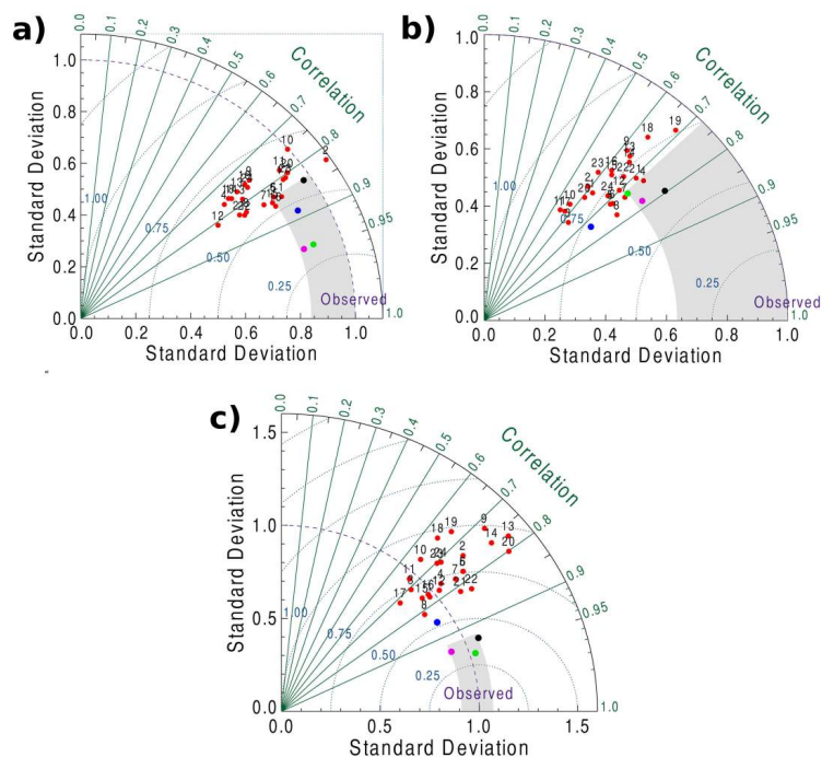
Fig. 14 Taylor diagrams for mean annual precipitation (a), relative entropy (b) and seasonality index (c). CMIP5 models are numbered as in Table 1. The MME, CRU, GPCP and CMAP are represented by the blues, black, green and magenta dots respectively. GPCC is taken as reference and standard deviations are normalized with respect to GPCC. The grey shaded areas are indicative of the range of observational uncertainty. The correlation analysis is restricted to land.
