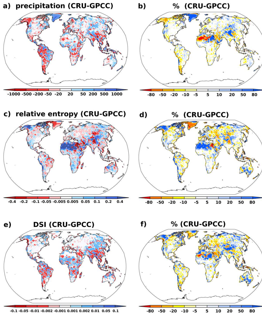
Fig. 4 Differences (a, c, e) and relative differences (b, d, f) between the CRU and the GPCC datasets for the same quantities in Fig. 1 over the period 1950-2010.
