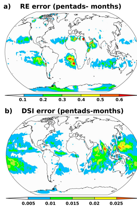
Fig. 3 Difference between the RE (a) and the DSI (b) estimated from pentad and monthly means.
