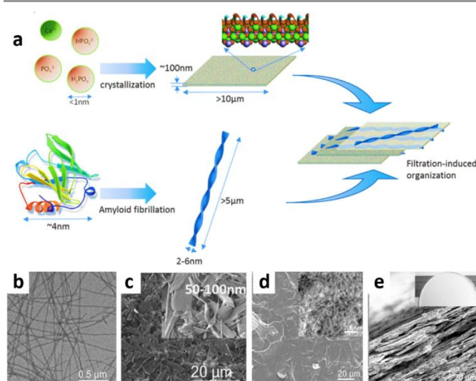
Fig. 23 (a) Schematic representation of the fabrication of bone-mimetic composites based on amyloid fibril and HA platelets. (b) TEM image of \beta -lactoglobulin amyloid fibrils. (c-e) SEM image of HA platelets (c), surface (d) and fracture sections (e) of the amyloid-based composite with 60 wt% brushite platelets. Reproduced with permission from Ref. 383. Copyright 2014, Wiley-VCH Verlag GmbH & Co.
