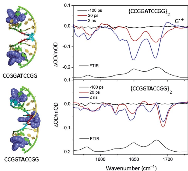
Fig. 19 TRIR spectra of \Delta -[Ru(TAP) 2 (dppz)] 2+ bound to d(CC GGATCC GG) 2 and d(CC GGTACC GG) 2 recorded at 20 ps and at 2 ns after 400 nm excitation. 67
