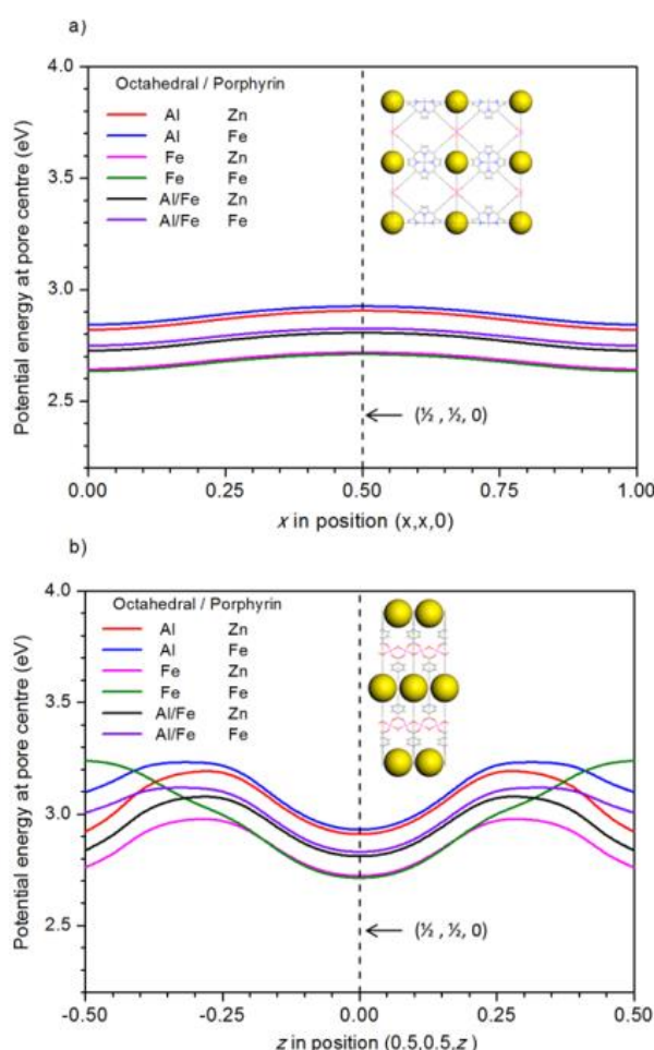
Figure 3. Electrostatic potential energy at the pore centre, as calculated with HSE06 functional along a) pores perpendicular to the porphyrin planes (coordinates (x,x,0) in the primitive cell), and b) pores parallel to the porphyrin plane (coordinates (0.5,0.5,z) in the primitive cell). The vertical dashed line in both figures corresponds to (0.5, 0.5, 0) , which is the point farthest apart from all atoms in the structure and is used to estimate the vacuum potential in this work. It is represented as large yellow spheres within the PMOF structures in the inset figures (shown in the conventional cell for clearer visualisation).
