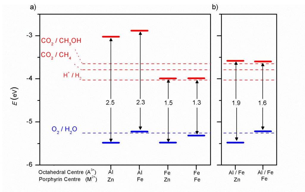
Figure 4. Band gaps and band edge positions with respect to the vacuum level, as calculated with the screened hybrid functional HSE06 for a) PMOF with only one element ( A = Al or Fe ) in the octahedral sites, and b) mixed PMOF with 50% Al and 50% Fe at the octahedral sites. The energy levels corresponding to redox potentials of water splitting and carbon dioxide reduction reactions producing methane and methanol at pH = 7 are also shown with dotted lines.
