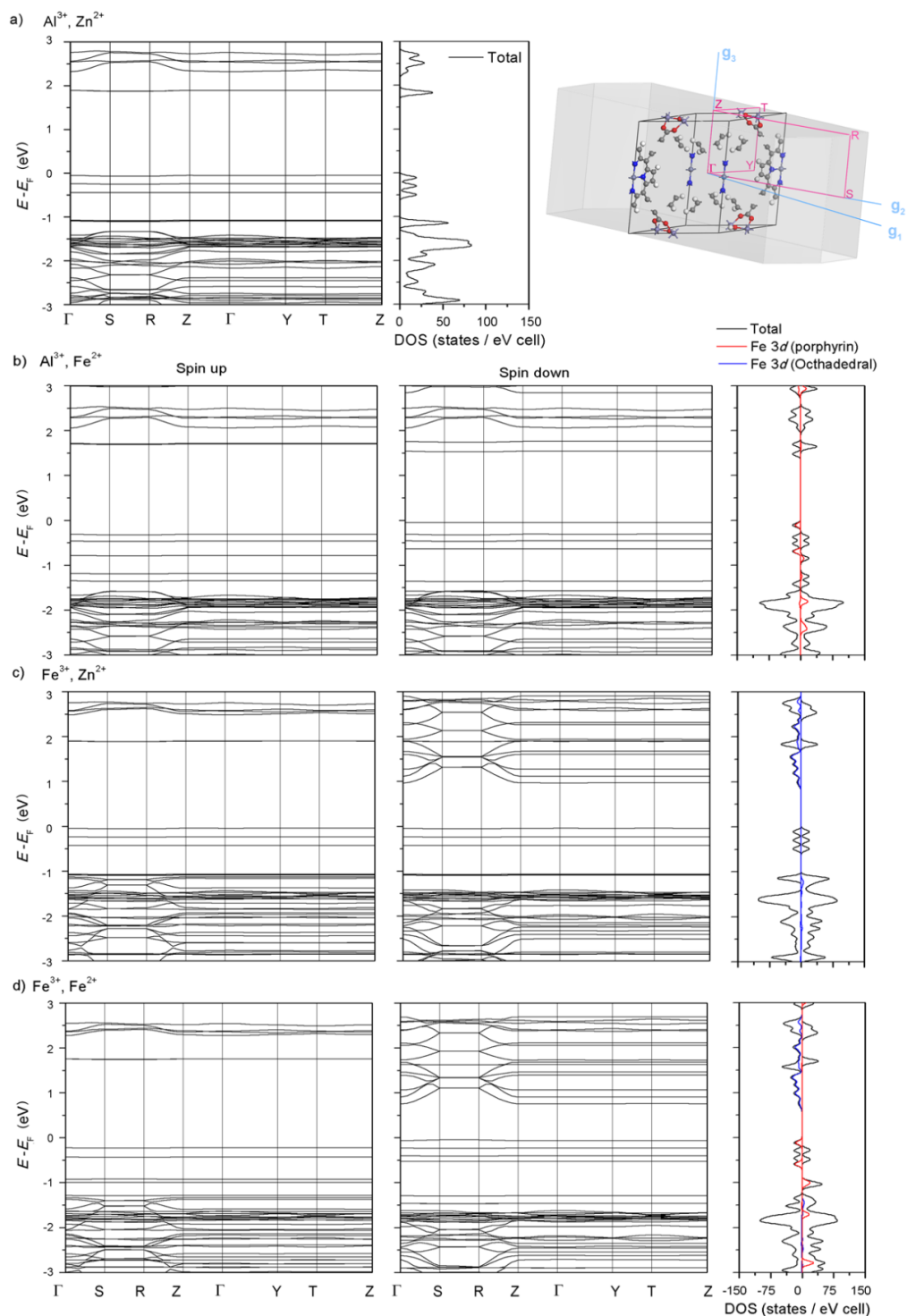
Figure S1: Electronic band structures and density of states (DOS) calculated using the PBE+U method for a) the “parent” structure (\text{Al}^{3+}, \text{Zn}^{2+})\text{PMOF} ; b) for the structure with Fe in the porphyrin metal centres, (\text{Al}^{3+}, \text{Fe}^{2+})\text{PMOF} ; c) for the structure with Fe in the octahedral metal centres, (\text{Fe}^{3+}, \text{Zn}^{2+})\text{PMOF} ; and d) for the structure with Fe both in the porphyrin and the octahedral metal centres, (\text{Fe}^{3+}, \text{Fe}^{2+})\text{PMOF} .
