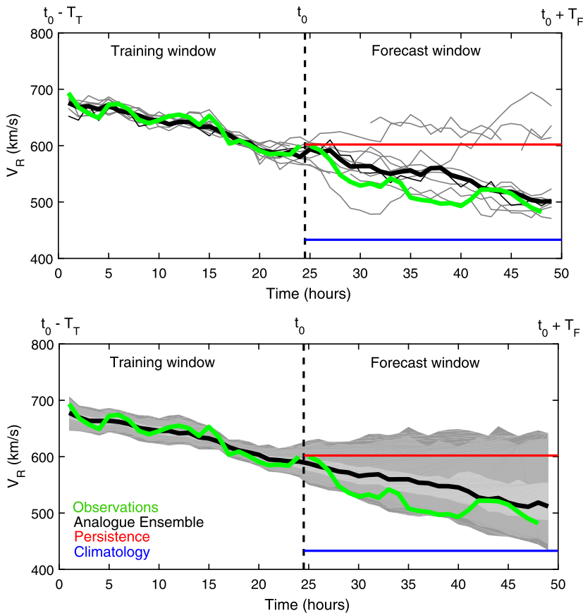
Figure 1 An example of an analogue ensemble (AnEn) for radial solar-wind speed [ V_R ]. The forecast is made at t_0 = 0:00 UT on 11 June 2003. The training window length [ T_T ] and the forecast window length [ T_F ] are both 24 hours. The solid green line shows the observed variation. The thin grey lines in the top panel show the ten closest analogues in the whole OMNI dataset to the observed variation in the training window. The thick black line shows the median of this ten-member ensemble. The grey shaded regions in the bottom panel show the bands containing 68%, 90%, and 95% of a 100-member ensemble. The red and blue lines show the persistence and climatological forecasts, respectively.
