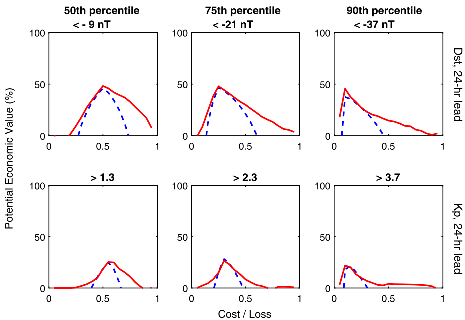
Figure 7 The potential economic value of a forecast (relative to climatology) for a range of cost/loss ratios, where cost is the expense of taking mitigating action and loss is the expense of not taking action during adverse space-weather conditions. Red lines show the AnEn, blue dashed lines show persistence. The top row shows the Dst forecast, the bottom row the Kp forecast. The columns show from left to right an increasing threshold for taking action, namely the 50th, 75th, and 90th percentile of the forecast parameter.
