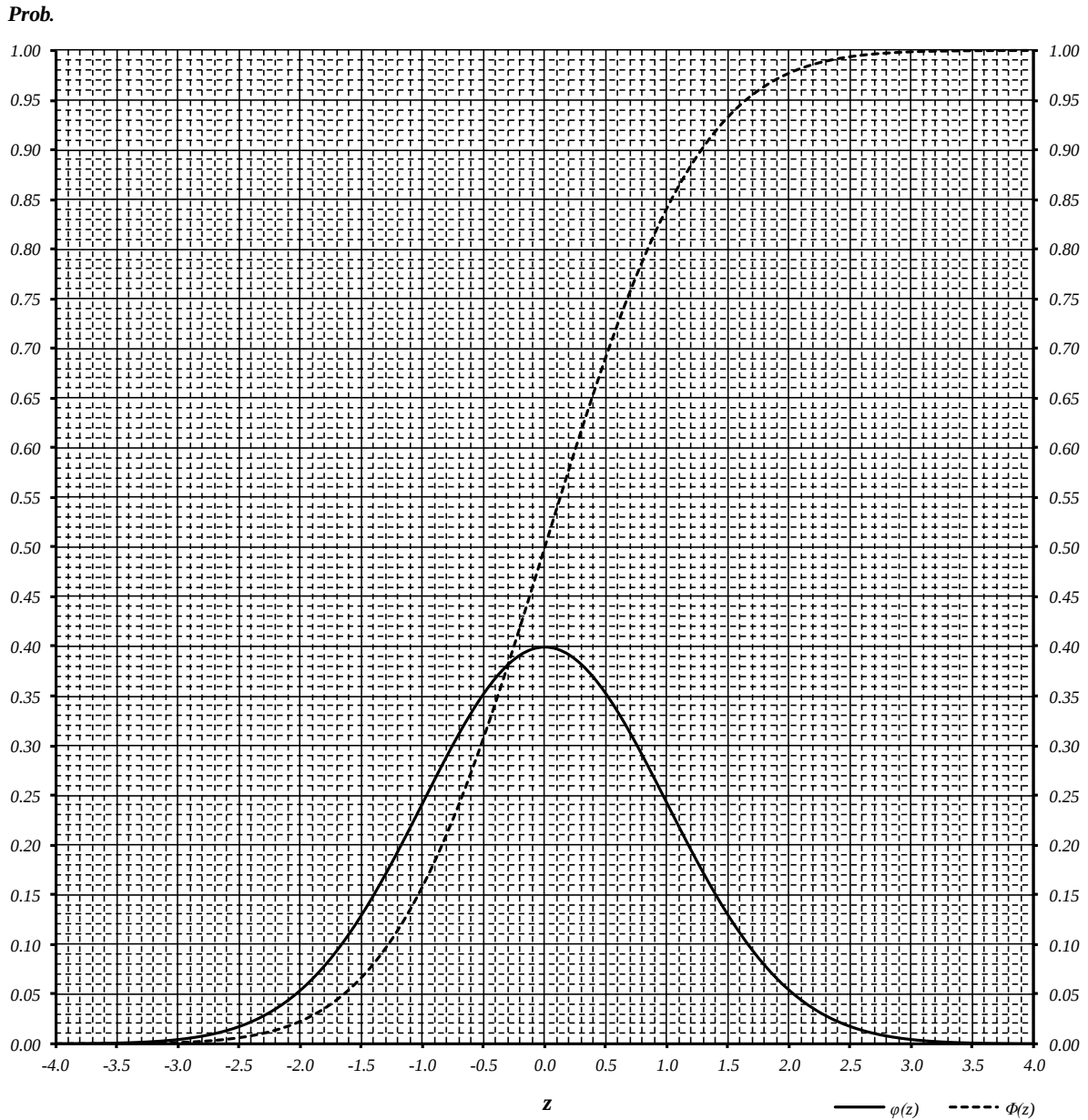
Supplemental Figure 1. Abacus for calculating the probability density function \phi(z) and the cumulative distribution function \Phi(z) of the Standard Normal distribution
