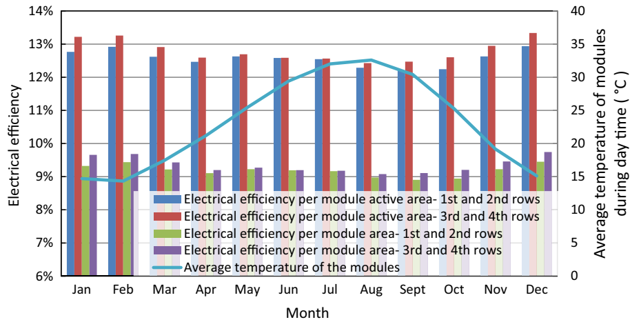
Fig. 16. Electrical efficiency per module area and the average temperature of the c-Si PV modules on southeast facing façade of the building at Yasar University campus, Izmir, Turkey.
