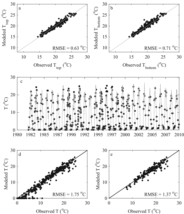
Fig. 3 Comparison of modelled and observed a surface and b bottom water temperatures for 2013–2015. c Comparison of long-term modelled (grey line) and observed (black dots) lake surface water temperature, showing a comparison d throughout the year and e during spring/summer (MJJA)
