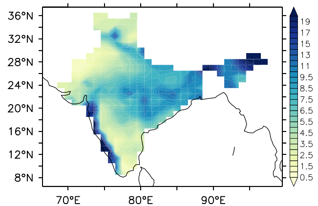
Fig. 2. June–September (JJAS) rainfall climatology ( \text{mm/day} ) during the period 1970–2000 from the India Meteorological Department (IMD) daily gridded observational dataset. Mean precipitation is highest over south-west peninsular India, north-east India and central India.
