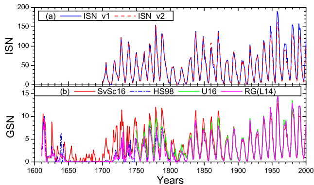
Figure 1. Temporal variation of the yearly means of the different reconstructions of SN series: Panel (a): ISN versions 1 (ISN_v1) and 2 (ISN_v2). Panel (b): the GSN by SvSc16 (red curve), by HS98 (blue dot–dashed curve), by Usoskin et al. (2016a) (U16, green curve) and by L14b (magenta curve).
