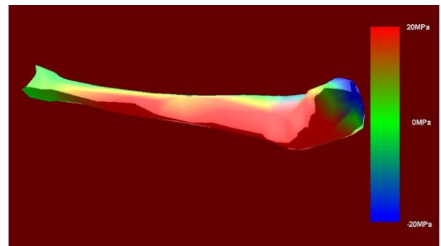
Fig 5. The regions of the tibia that are above 20 MPa threshold are shown in red. Here the gluteus maximus (biomechanically simulated) and quadriceps were both active bilaterally during in the drive phase of rowing. This suggests that supra-threshold stress extends further distally than for the 4-Ch case in figure 2.
