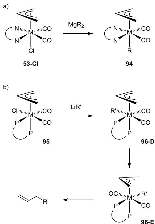
Scheme 32. Comparison between the reactions of non-stabilised carbanions ( R = \text{methyl, ethyl, benzyl} ) with \alpha -diimine complexes 94 ( M = \text{Mo, W} ; N\wedge N = \text{bpy, phen} ), and that of the molybdenum and tungsten dmpm congeners 95 ( R' = \text{Ph, } -\text{C}\equiv\text{CPh, 2-furyl, 2-thienyl} ). C–C coupling via an intramolecular migration is only observed for the latter, while 94 is not able to isomerise such that the coordinated carbanion becomes cis to the allyl ligand. [240]
