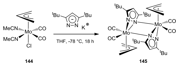
Scheme 48. Reaction of complex 144 with the potassium salt of 3,5- t -butylpyrazolate. [322]
