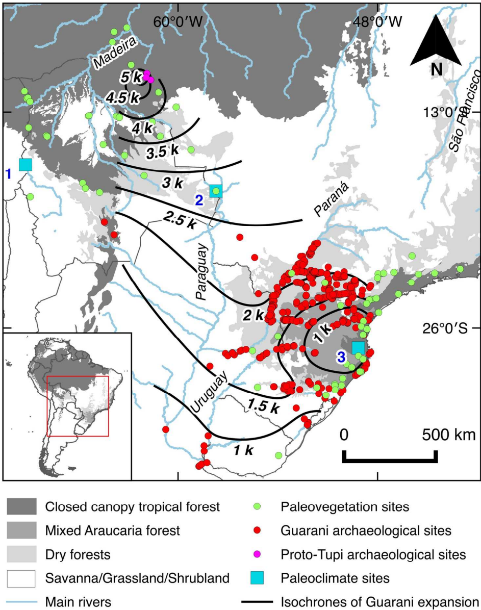
Figure 1. Map of study area showing locations of 1181 Guarani and Proto-Tupi archaeological sites (see Tables S1 and S2, available online), palaeoecological sites (see Table S6, available online) and palaeoclimate sites, including: 1. Lake Titicaca; 2. Laguna La Gaiba; and 3. Botuverá Cave (Section S2, available online). Isochrones show the time-transgressive movement of the Guarani culture (k = k yr B.P.). 144x183mm (300 x 300 DPI)
