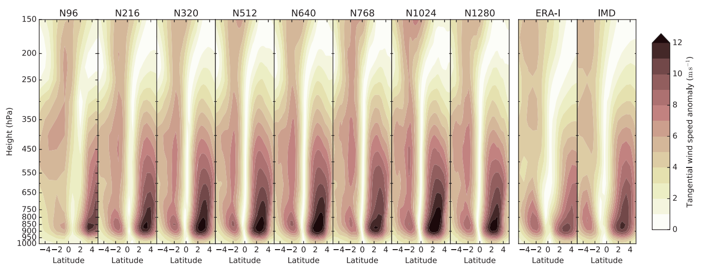
Figure 14. Mean composite wind speed anomaly ( \text{m s}^{-1} ) for the case-study MDs. Construction of the composite is as Figure 11 and the anomaly is taken against the climatology, whose computation is as in Figure 13.
