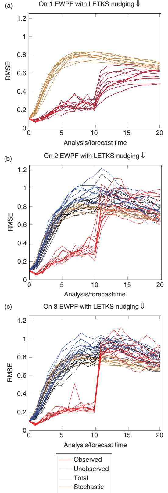
Fig. B4. Performance of the EWPF with the LETKS relaxation when \kappa = 0.25 .
