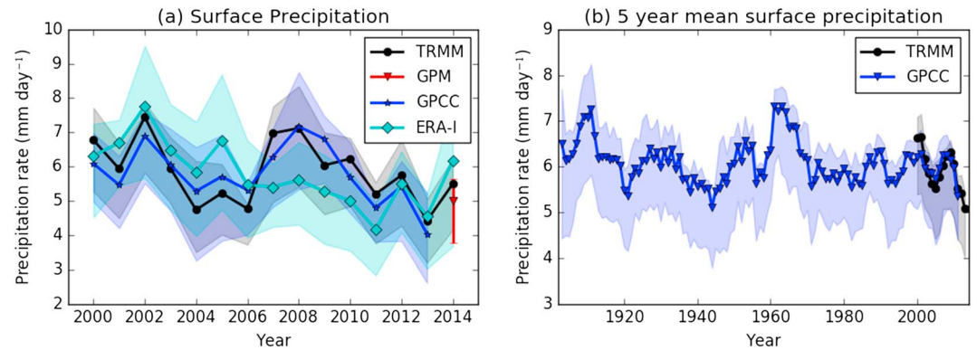
Figure 3. June–July mean precipitation ( \text{mm d}^{-1} ). (a) June–July means for individual years as observed by TRMM, GPM, and GPCC and modeled in ERA-Interim. (b) Five year running means for June–July for TRMM and GPCC. The shaded regions (error bar for GPM) shows spatial variability, indicated by the interquartile range over the DACCWA region, based on 1^\circ resolution.
