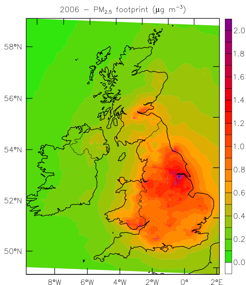
Fig. 2 Annual average regional PM 2.5 concentrations (µg m -3 ) from major industrial source regulated in the UK in 2006
