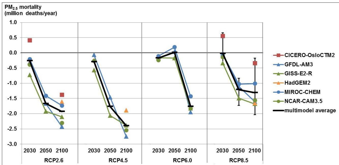
Figure 4: Estimates of future premature mortality (IHD+STROKE+COPD+LC) for PM_{2.5} calculated as a sum of species, for all RCP scenarios in 2030, 2050 and 2100, showing global mortality for six models and the multi-model average (million deaths/year), for future air pollutant concentrations relative to 2000 concentrations. Uncertainty shown for the RCP8.5 multi-model average is the 95% CI including uncertainty in RR and across models.
