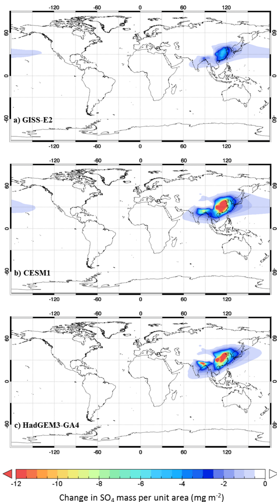
1 2 Figure 3: Global changes in column-integrated \text{SO}_4 burden due to removing anthropogenic \text{SO}_2 3 emissions from China, for a) GISS-E2, b) CESM1, and c) HadGEM3-GA4. Differences are 4 calculated as perturbation simulation minus control simulation, averaged over 150 years.
