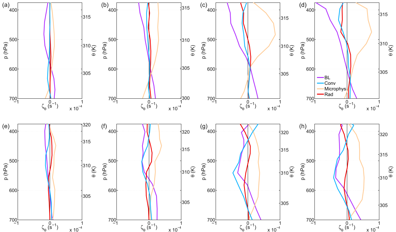
FIG. 13. Vertical profiles of contributions of BL and turbulent mixing processes (BL), parameterized convection (Conv), cloud microphysics processes (Microphys), and radiation (Rad) to average isentropic vorticity for a 500-km spherical cap concentric to the cyclone for (a)–(d) IOP13 and (e)–(h) IOP14: (a) 1500 UTC ( T + 3 ) and (b) 2100 UTC 17 Jul 2012 ( T + 9 ); (c) 0300 UTC ( T + 15 ) and (d) 0900 UTC 18 Jul 2012 ( T + 21 ); (e) 2100 UTC 14 Aug 2012 ( T + 3 ); (f) 0300 UTC ( T + 9 ); (g) 0900 UTC ( T + 15 ); and (h) 1500 UTC 15 Aug 2012 ( T + 21 ).
