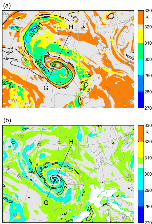
FIG. 7. As in Fig. 4, but for IOP14 at 1500 UTC 15 Aug 2012 ( T + 21 ) at the isentropic levels (a) 320 and (b) 305 K. The segment G–H indicates the position of the vertical sections in Figs. 8 and 9. WCB1 and WCB2 indicate the primary and secondary WCB branches, respectively.
