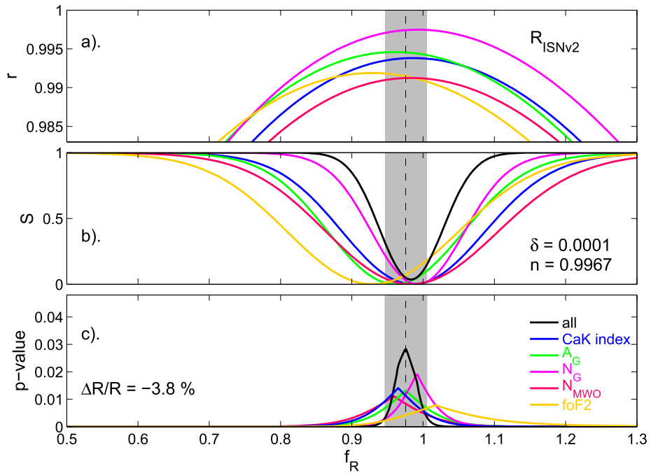
Figure 6 Same as Figure 5 for Version 2 of the of the Wolf/Zürich/International sunspot number [ R_{\text{ISNV2}} ]. (a) The correlation [ r ] as a function of the factor f_R of the adjusted sequence [ R_{\text{ISNV2}}' ] (generated using Equation (1) before 1946 where the tested parameter R is R_{\text{ISNV2}} ) with (mauve) the RGO group-number [ N_G ], (green) the corrected RGO total-spot-area number [ A_G ], (blue) the Mount Wilson CaKi index, and (orange) the F2 layer critical frequency at Slough [foF2]. (b) The significance [ S ] of the differences between the peak r and the r at general f_R (using the same colour scheme). The black line is the combination of the four S(f_R) variations using Equation (3). (c) The p -values of the difference in the mean residuals between the “before” (1932–1943) and “after” (1949–1960) intervals [ p(f_R) ], again using the same colour scheme. The black line is the combination of the four pdfs [ p(f_R) ] made using Equation (2). The vertical-dashed line marks the peak, and the grey area the range between the 2\sigma points, of the combined p(f_R) . The plot is for the optimum offset value [ \delta ] of 1.4938 \times 10^{-4} and exponent [ n ] of 0.9967 (see Table 3).
