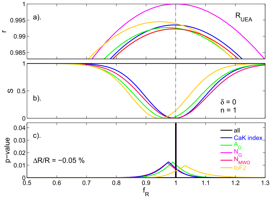
Figure 9 Same as Figure 5 for the new Usoskin et al. (2015) group-number reconstruction [ R_{\text{UEA}} ]. (a) The correlation r as a function of the factor f_R of the adjusted sequence [ R_{\text{UEA}}' ] (generated using Equation (1) before 1946 where the tested parameter R is R_{\text{UEA}} ) with (mauve) the RGO group number [ N_G ], (green) the corrected RGO total spot area number [ A_G ], (blue) the Mount Wilson CaKi index, and (orange) the F2 layer critical frequency at Slough [foF2]. (b) The significance [ S ] of the differences between the peak r and the r at general f_R (using the same colour scheme). The black line is the combination of the four S(f_R) variations using Equation (3). (c) The p -values of the difference in the mean residuals between the “before” (1932–1943) and “after” (1949–1960) intervals [ p(f_R) ], again using the same colour scheme. The black line is the combination of the four pdfs [ p(f_R) ] made using Equation (2). The vertical-dashed line marks the peak, and the grey area the range between the 2\sigma points, of the combined p(f_R) . The plot is for the optimum offset value [ \delta ] of 0 and exponent [ n ] of 1 (see Table 3). Note that [ p(f_R) ] N_G and hence p(f_R) are very close to \delta -functions in this case (they are not quite because the other test series are not quite identical in waveform to N_G ) and although part c uses the same p(f_R) scale as Figures 3–6, the peak p(f_R) value [ p_m ] is close to unity.
