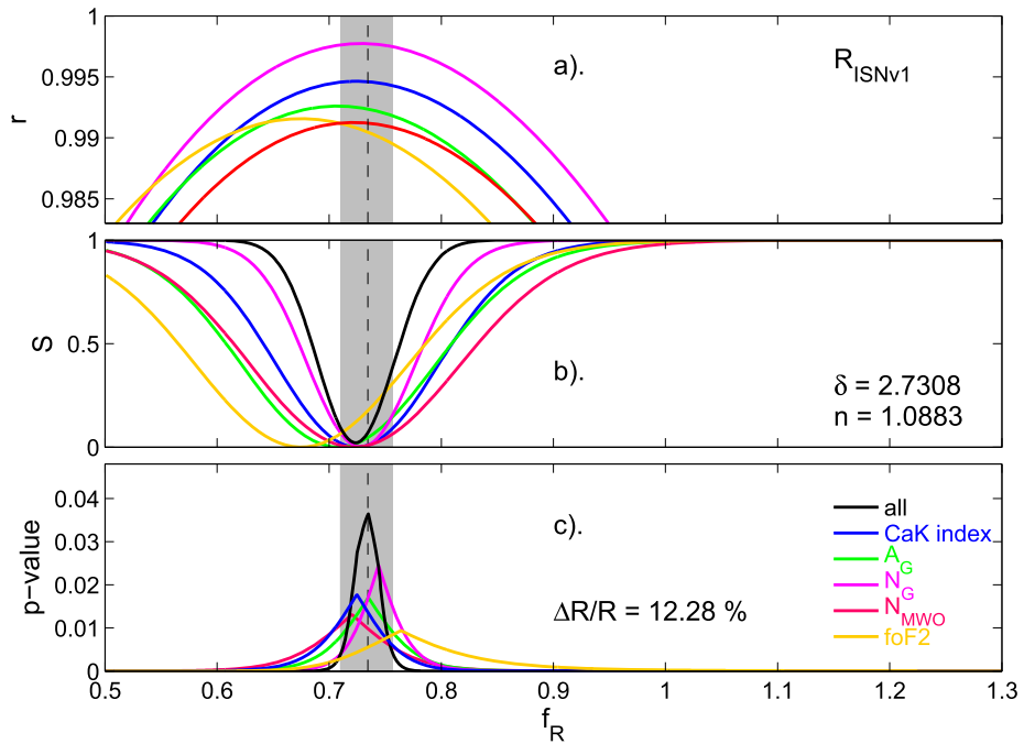
Figure 5 Evaluation of the discontinuity around 1946 for Version 1 of the Wolf/Zürich/International sunspot number [R_{\text{ISNV1}}] . (a) The correlation r as a function of the factor f_R of the adjusted sequence [R_{\text{ISNV1}}'] (generated using Equation (1)) before 1946 where the tested parameter R is R_{\text{ISNV1}} with (mauve) the RGO group-number [N_G] , (green) the corrected RGO total-spot area-number [A_G] , (blue) the Mount Wilson CaKi index, and (orange) the F2 layer critical frequency at Slough [foF2]. (b) The significance [S] of the differences between the peak r and the r at general f_R (using the same colour scheme). The black line is the combination of the four S(f_R) variations using Equation (3). (c) The p -values of the difference in the mean residuals between the “before” (1932–1943) and “after” (1949–1960) intervals [p(f_R)] , again using the same colour scheme. The black line is the combination of the four pdfs [p(f_R)] made using Equation (2). The vertical-dashed line marks the peak, and the grey area the range between the 2\sigma points, of the combined p(f_R) . The plot is for the optimum offset value [\delta] of 2.7309 and exponent [n] of 1.0884 (see Table 3).
