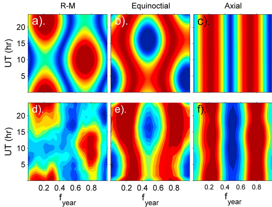
Figure 2. Predicted and observed time-of-day/time-of-year patterns. (a–c) Predictions based on geometric factors and (d–f) the contoured patterns in means of observations. (Figure 2a) the Russell-McPherron (R-M) pattern: The filled color contours show |\sin(\delta_a + \delta_d)| (see Figure 1) as a function of fraction of the year, f_{\text{year}} , (horizontal axis) and UT (vertical axis). (Figure 2b) The equinoctial pattern, shown by \cos(\psi) where \psi is the full angle between the Earth's magnetic dipole axis, M , and the GSE X axis. (Figure 2c) An axial pattern shown by |\sin(\Lambda_E)| , where \Lambda_E is the heliographic latitude of Earth. (Figure 2d) The pattern for the mean of the observed southward IMF in GSM coordinates, B_S(\text{GSM}) , where B_S(\text{GSM}) = -B_Z(\text{GSM}) when B_Z(\text{GSM}) < 0 and B_S(\text{GSM}) = 0 when B_Z(\text{GSM}) \geq 0 . (Figure 2e) The pattern for the a_m geomagnetic index. (Figure 2f) The pattern for -k(\text{UT}) \times Dst where the factor k(\text{UT}) is the modeled response of the four Dst stations that allows for the fact that they are not equally spaced in longitude (see section 3.1 of text). To get good coverage, all available data were used in each case, namely, 1963–2015 for the IMF data in Figure 2d; 1959–2015 for the a_m data in Figure 2e; and 1957–2015 for the Dst data in Figure 2f. In all cases we are concerned only with the form of the pattern rather than the amplitude and color scales have been autoscaled between the maximum and minimum values.
