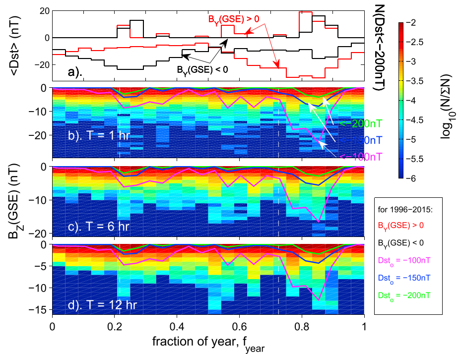
Figure 7. (a) The mean Dst and the number of hours of Dst below the threshold Dst_0 of -200 nT, N(Dst < -200 \text{ nT}) as a function of t-o-y ( f_{\text{year}} ): red/black lines are for when the mean IMF B_y(\text{GSE}) in the previous 12 h was positive/negative, respectively. Negative values are \langle Dst \rangle , positive values are N(Dst < -200 \text{ nT}) . (b, c, and d) The occurrence of southward IMF B_z(\text{GSE}) as a function of time-of-year, f_{\text{year}} , for averaging timescale T of (1) 1 h, (2) 6 h, and (3) 12 h. The number of samples, N , in 1 nT bins of B_z(\text{GSE}) and (1/24) bins of f_{\text{year}} is shown, normalized to the total number for that f_{\text{year}} bin, \Sigma N . Note that each pixel is colored on a logarithmic scale of N/\Sigma N . By using a maximum of zero on each B_z(\text{GSE}) axis, the plots show only the results for southward IMF. Note also that different B_z(\text{GSE}) scales are used for the three panels because the distributions are narrower for larger T . Each panel also shows the number of hours, times a negative constant ( c < 0 ), of Dst < Dst_0 for thresholds of (mauve line) Dst_0 = -100 nT, (blue line) Dst_0 = -150 nT, and (green line) Dst_0 = -200 nT. The value of c is different in the three panels and c is negative to make visual comparison with the B_z(\text{GSE}) occurrence easier. Vertical dashed white lines mark the equinoxes.
