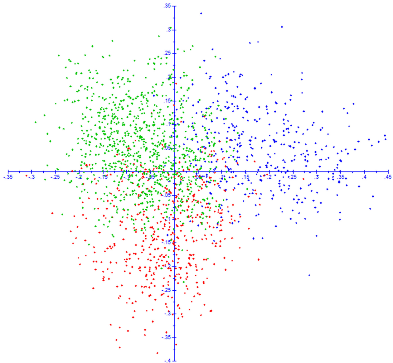
Fig. 2 Scatter plot of the Principal Coordinate Analysis (PCoA) of the 1859 apple accessions based on the 16 SSR data. The three groups are depicted using the following color codes: Red = group K1; Blue = group K2; Green = group K3
