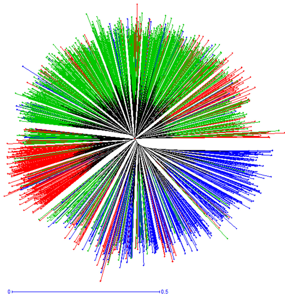
Fig. 3 Neighbor-joining dendrogram based on simple matching dissimilarity matrix calculated from the dataset of 16 SSR markers for the 1859 genotypes clustered in the three groups revealed by the Bayesian model-based clustering method. The three groups are depicted using the following color codes: Red = group K1; Blue = group K2; Green = group K3
