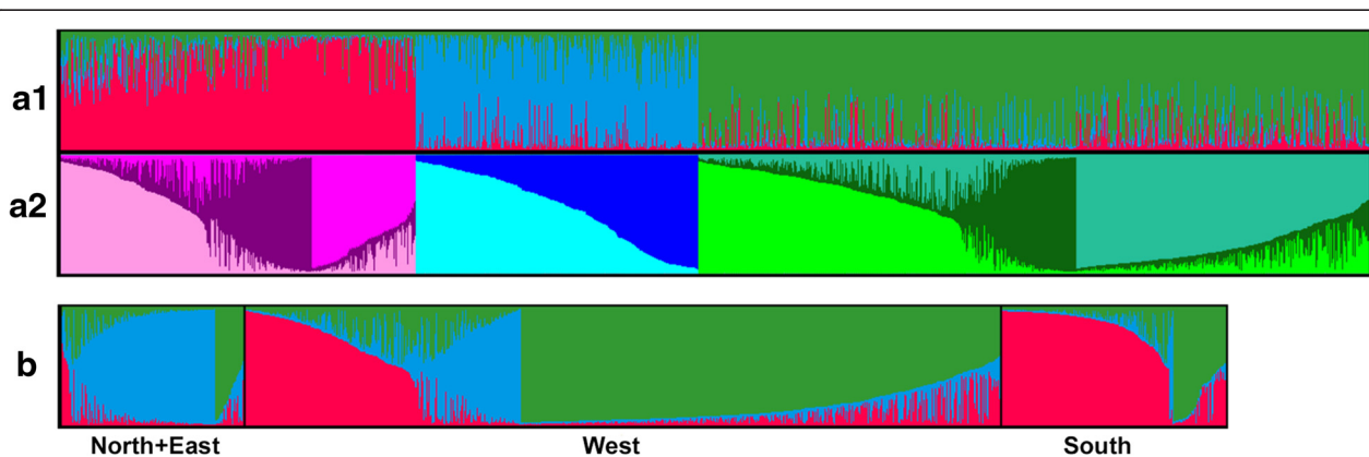
Fig. 1 Graphical display of the results of the Structure analyses. a1 ) Proportions of ancestry of 1859 unique diploid apple genotypes for K = 3 groups inferred with Structure v.2.3.4 software [67]. Each genotype is represented by a vertical bar partitioned into K = 3 segments representing the estimated membership fraction in three groups. The three groups are depicted using the following color codes: Red = group K1; Blue = group K2; Green = group K3. a2 ) Proportions of ancestry of the same 1859 genotypes following a nested Structure analysis within each previously defined group. For K1 and K3 three subgroups are shown and for K2 two subgroups are shown. Each genotype is represented by a vertical bar partitioned into K = 2 or 3 subgroups representing the estimated membership fraction in each subgroup. Genotypes are presented in the same order than in a1. The subgroups are depicted using the following color codes: light Pink = K1.1; Purple = K1.2; dark Pink = K1.3; light Blue = K2.1; dark Blue = K2.2; fluorescent Green = K3.1; dark Green = K3.2; light Green = K3.3. b ) Proportions of ancestry of 1653 unique diploid apple genotypes with known European region of origin for K = 3 groups inferred with the same Structure analysis as in a. The genotypes are sorted according to their European region of origin (North + East, West, and South)
