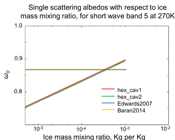
Fig. 13. Single scattering albedos plotted against ice mass mixing ratio, as predicted by hex_cav, Edwards2007 and Baran2014 at T = 270 K.
