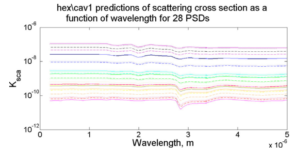
Fig. D.23. Bulk K_{\text{sca}} values calculated using the hex_cav1 parameterization. Each trace represents a different PSD from Field2007.
