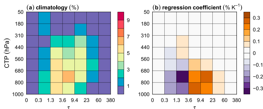
Figure 3. ISCCP cloud fraction histograms binned by cloud top pressure (CTP) and optical depth ( \tau ). (a) Mean climatology and (b) regression coefficient on low-level temperature, both averaged over the 45°–60°S latitude range.
