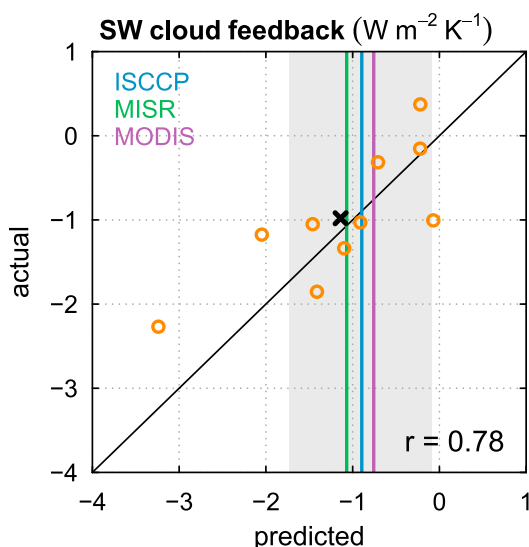
Figure 5. Scatterplot of actual versus predicted SW cloud feedback, averaged over 45^{\circ} – 60^{\circ} S. Vertical colored bars denote the predictions associated with satellite observations. Grey shading represents the 95% uncertainty interval for the mean of the three observational estimates (Text S3). The black cross marks the multimodel mean. The orange open circles are as in Figure 2.
