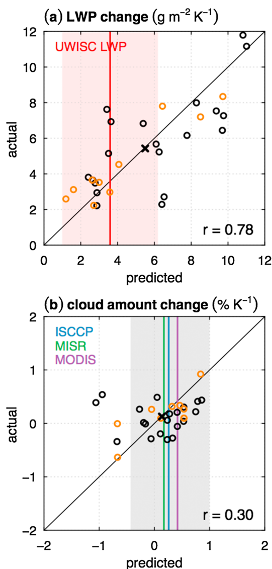
Figure 2. Scatterplots of actual versus predicted (a) LWP change and (b) cloud amount change, both averaged over 45^{\circ} – 60^{\circ}\text{S} . The black crosses mark the multimodel mean. Vertical colored bars denote the predictions associated with observational data sets, and orange open circles indicate the models with cloud property histogram data that were used for the SW cloud feedback calculation in Figures 4 and 5. Shading represents the 95% uncertainty interval for the mean observational estimates, calculated as described in Text S3.
