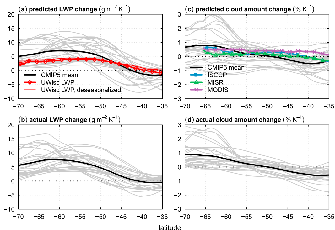
Figure 1. Predicted and actual change in liquid water path (LWP) and cloud amount in CMIP5 models and in observations. (a, c) The predicted changes are based on regressions onto low-level (500–850 hPa) temperature (see section 2); (b, d) the actual changes are calculated as 2081–2100 minus 1981–2000 in the RCP8.5 experiment, normalized by the low-level temperature change in each model. Observed cloud amount is obtained by integrating the cloud property histograms over all cloud top pressure and optical depth bins. Grey curves denote individual models, the thick black curve represents the multimodel mean, and colored curves correspond to observational data sets. For observations, pale color shading denotes the 95% confidence intervals based on a two-sided significance test for the regression slope; these confidence intervals are often not visible due to their narrowness.
