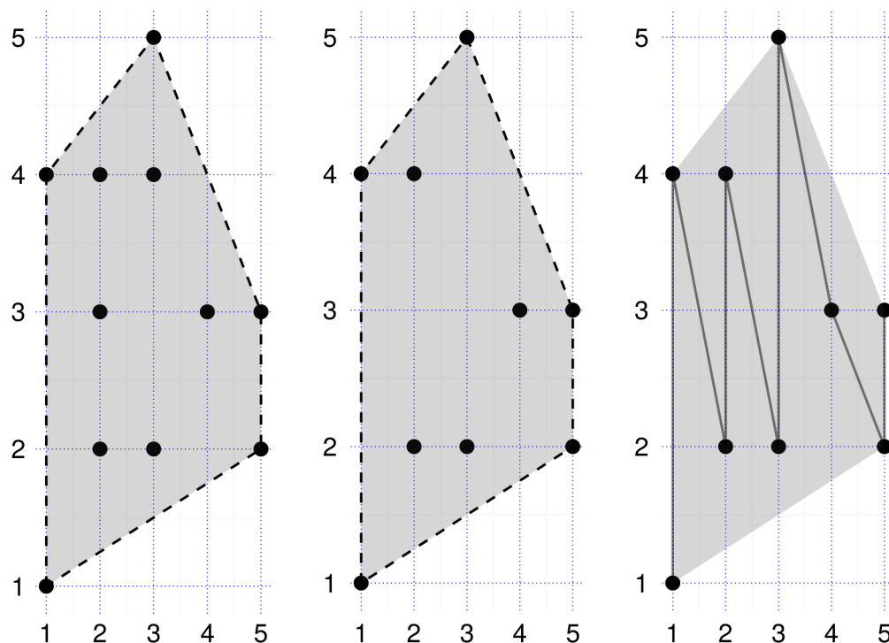
Fig 1. A small example of 2D points with integer coordinates. Left: (x, y) integer points on a 2D grid with p = 5 . Center: Points with minimum and maximum y values for each x coordinate. Right: A polyline.
