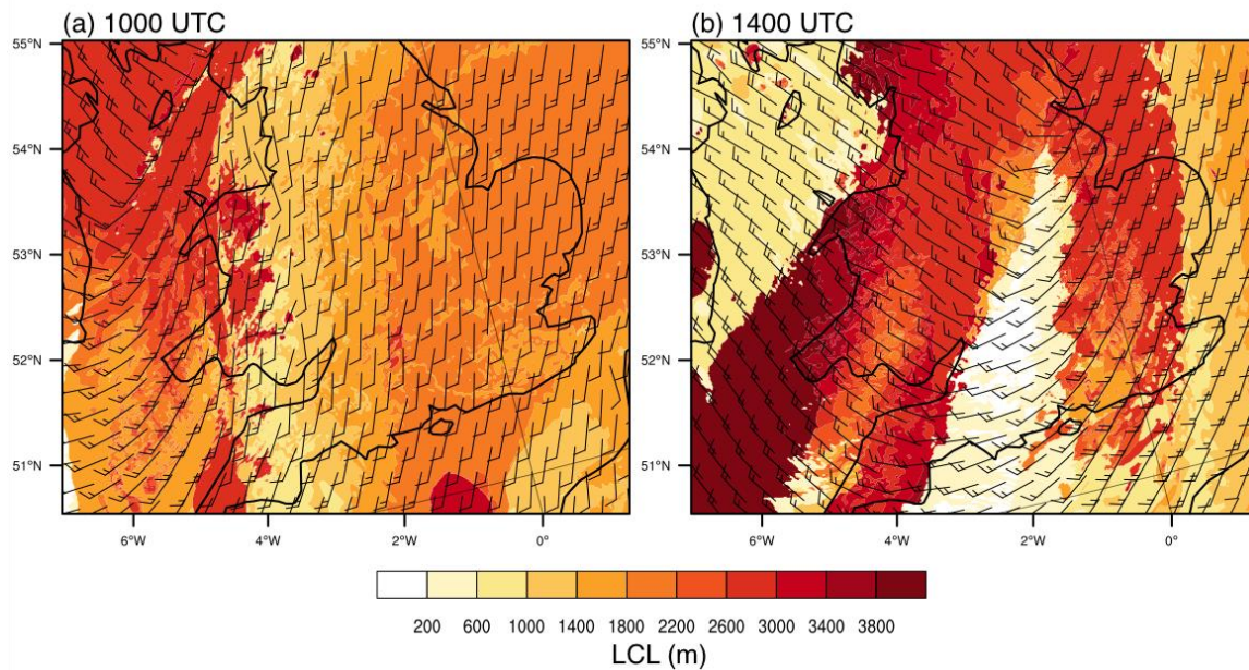
Figure 14. Simulation of lifting condensation level (LCL) (m, colored according to scale) and surface winds (pennant, full barb, and half-barb denote 25, 5, 2.5 m s -1 , respectively; separation between displayed wind vectors is 30 km) on the domain with 1-km horizontal grid spacing at (a) 1000 UTC and (b) 1400 UTC 23 November 1981.
