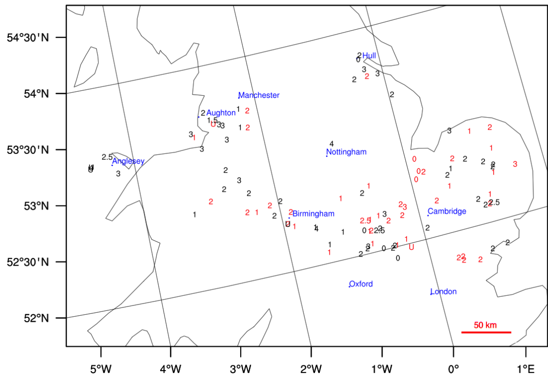
Figure 1. Locations of the 104 tornado reports from the TORRO database for 23 November
