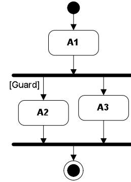
Figure 3. Activity Diagram
