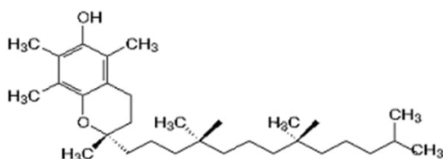
I Chemical structure of \alpha -tocopherol
