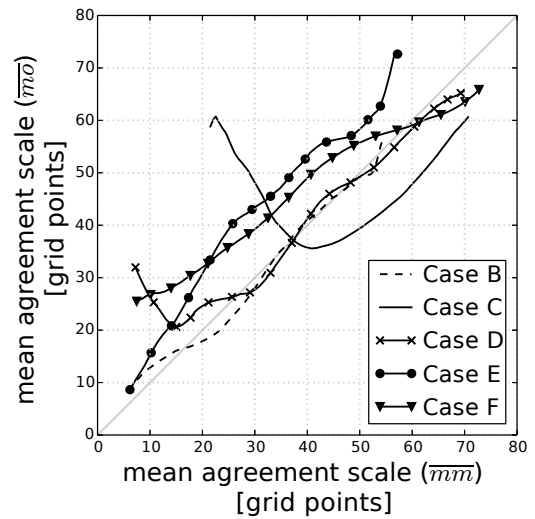
(b) 1300 UTC
