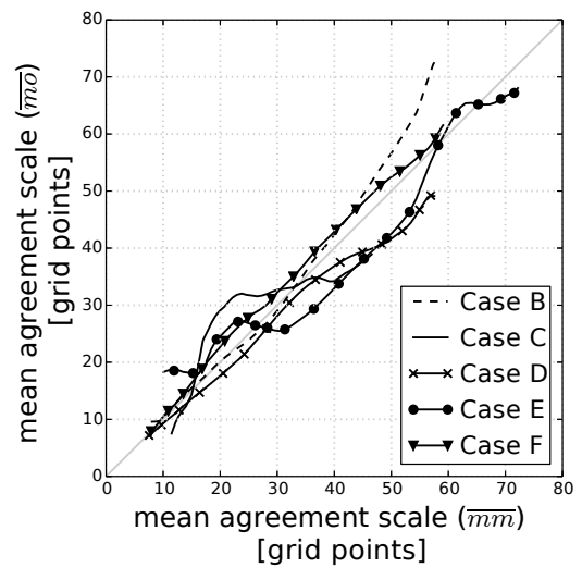
(c) 1700 UTC
