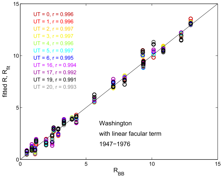
Figure 11 The same as Figure 9 for Washington foF2 data. Specifically, the values from the third-order-polynomial fits with a linear term in the white-light facular area [ R_{\text{fit}} ] are shown as a function of R_{\text{BB}} . The solid line is the ideal fit of slope unity and intercept zero. The colours give the UT and correlation coefficient for this UT. As for Figure 9, these data are from the interval 1947–1976.
