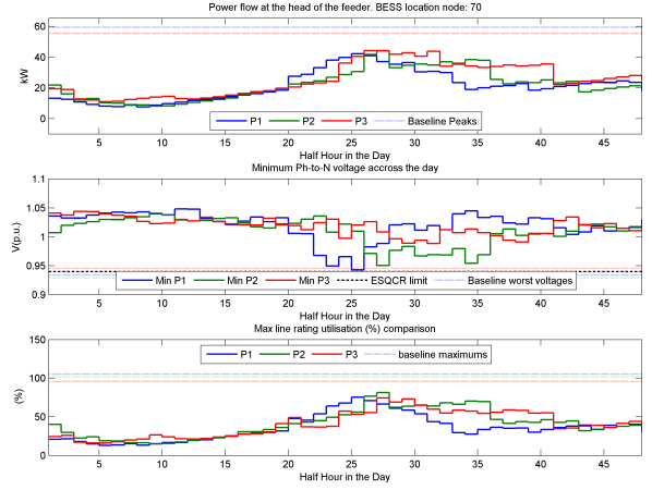
(b) Three-phase storage
