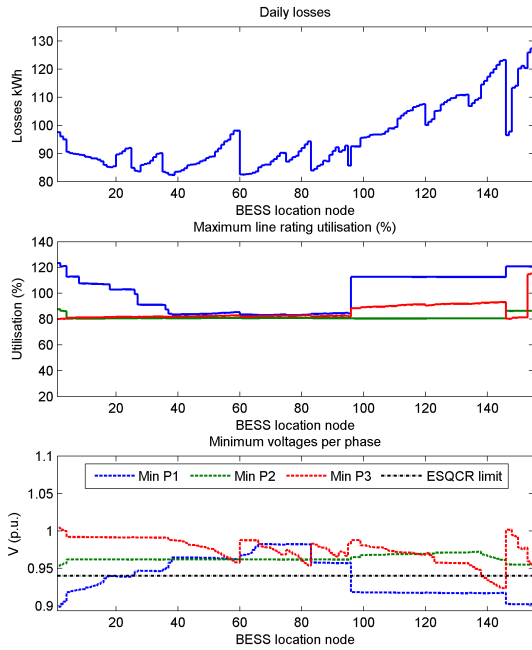
(c) Impact of Configuration 3 (three-phase phase-balancing BESS).
