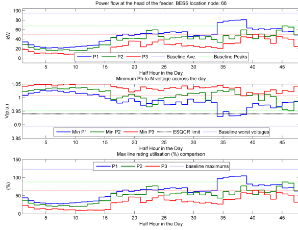
(a) Single-Phase Storage
