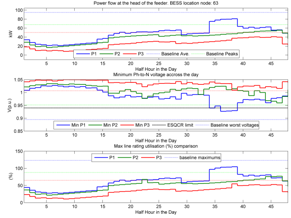
(b) Three single-Phase Storage
