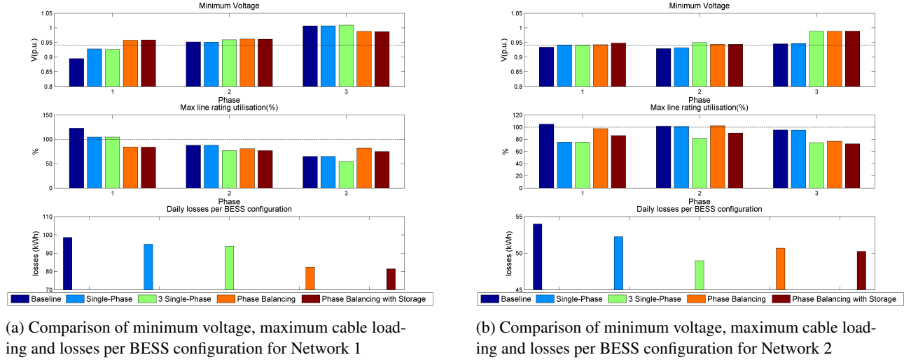
Figure 6: Summary of the impact of BESS locations.
