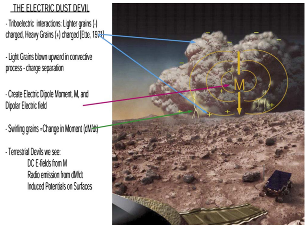
Fig. 3 An artist's impression of an electrified dust devil at Mars (from Farrell et al. 2004)
