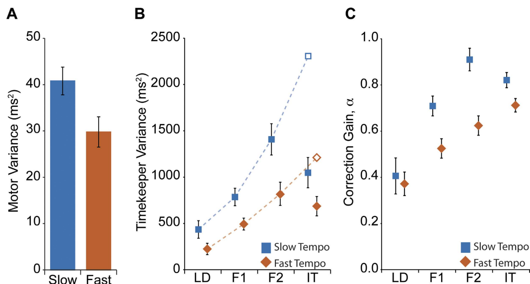
Figure 4. Parameters from a linear phase correction model were estimated from each participant's asynchrony and IMI time series data. (A) Motor Variance. Estimates of motor variance remained relatively constant across positions. However, movements in the slow tempo conditions showed higher motor variance compared to estimates from the fast tempo conditions. Error bars indicate SEM. (B) Timekeeper Variance. As with motor variance, timekeeper variance was higher at slow movement tempos (blue square markers) than for fast movement tempos (orange diamonds). Estimates of timekeeper variance also showed increasing values further along the chain, indicating sensitivity to higher cue variance generated by the adjacent position. Moreover, as observed for IMI variability, we saw no significant increase in timekeeper variance in position IT, with actual estimates (filled symbols) being much lower than the predicted value (open symbol marker). Dashed lines show polynomial fits (order 2) based on the points LD, F1 and F2 only. Error bars are SEM. (C) Correction Gain. Estimates of correction gain indicate that participants actually increased their corrections as they moved further down the chain. Additionally, correction gains were larger in the slow tempo (blue squares) than the fast tempo (orange diamonds) conditions. Once again, we observed evidence in a change of strategy in the IT position compared to the other positions in the chain. Error bars are SEM.
