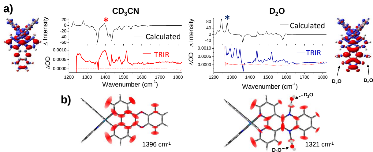
Fig. 7 a) Simulated difference spectra compared with the experimental TRIR spectra of 1 in acetonitrile (left column); and 1 ·2( \text{D}_2\text{O} ) in water (right column). In the experimental spectra, wavenumbers below 1250\text{ cm}^{-1} were inaccessible due to strong absorbance of both solvents in this region. Structural inserts show electron density difference map (iso level 0.0008) between the lowest energy triplet state of 1 minus the electron density of the equivalent singlet ground-state at the same geometry in acetonitrile (left hand side) and for 1 ·2( \text{D}_2\text{O} ) in water (right hand side). (The red and blue volumes indicate the regions where the electron density is respectively higher and lower in the triplet state compared to the ground state); b) Graphical illustration of the in-plane vibrational modes of the marker bands of the “bright” and “dark” states of 1 at 1396\text{ cm}^{-1} in \text{CD}_3\text{CN} and 1321\text{ cm}^{-1} in \text{D}_2\text{O} (marked with asterisks in the spectra). Red ellipsoids indicate the regions of largest atomic displacement. Animations of these vibrations can be found online in the ESI† (Animation 1- \text{CD}_3\text{CN} and Animation 2- \text{D}_2\text{O} ).
