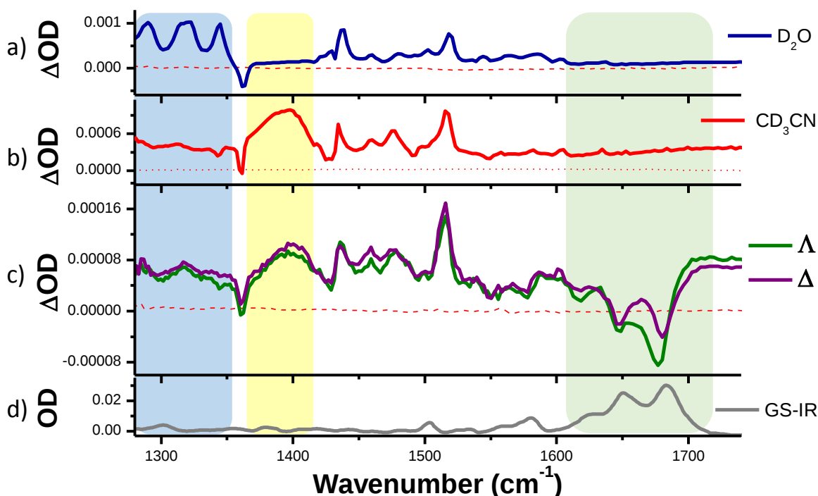
Fig. 8 TRIR spectra recorded 35 ps after 400 nm excitation of a) 1 ·2Cl (500 \mu M) in D_2O , b) 1 ·2PF 6 (500 \mu M) in CD_3CN and c) \Delta - and \Lambda -[ 1 ]2Cl (400 \mu M) and a duplex DNA oligonucleotide d(TCGGCGCCGA) 2 (500 \mu M duplex) and d) FTIR spectrum oligonucleotide d(TCGGCGCCGA) 2 (500 \mu M duplex) in deuterated potassium phosphate buffer (50 mM) pH 7. The blue and yellow coloured regions highlight the characteristic transient bands for the excited state of 1 , while the green coloured region highlights the bands associated with the base DNA base pairs.
