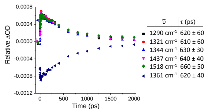
Fig. 5 ps-TRIR( \lambda_{ex} = 400 nm) decay kinetics of the transient bands at 1290, 1321, 1344, 1437 and 1518 cm^{-1} and bleach at 1361 cm^{-1} of 1-2Cl (500 \mu M ) in D_2O
