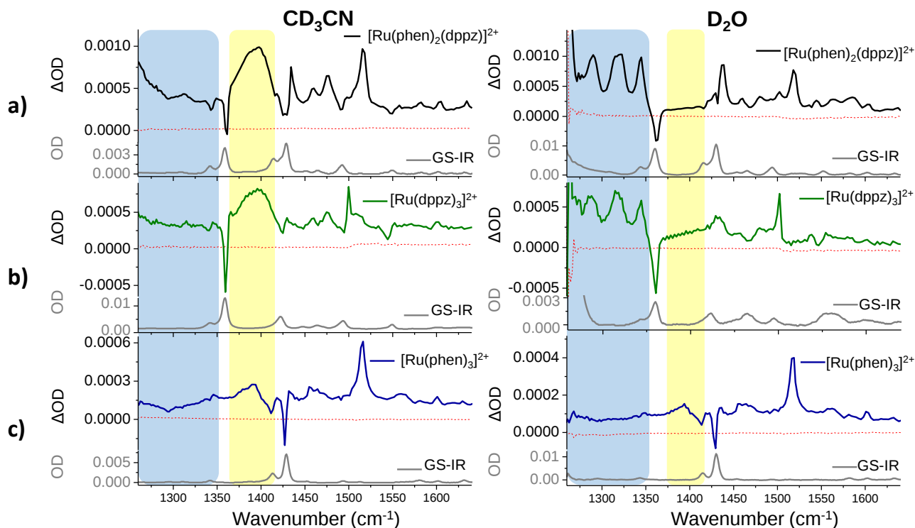
Fig. 4 Time-resolved infrared (TRIR) spectra recorded 35 ps after 400 nm excitation of 1 ·2PF 6 − (500 μM), 2 ·2PF 6 − (500 μM) and 3 ·2Cl − (500 μM) in CD 3 CN (left column) and of 1 ·2Cl − (500 μM), 2 ·2Cl − (300 μM) and 3 ·2Cl − (500 μM) in D 2 O (right column) and their corresponding ground state FTIR (GS-IR) spectra. The blue and yellow coloured regions highlight the characteristic transient bands for the “bright” and “dark” excited states. a, b and c refer to the TRIR spectra of complex 1 , 2 and 3 in both solvents.
