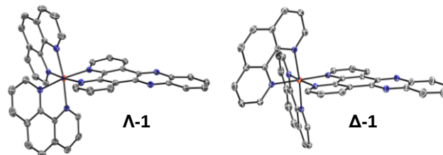
Fig.2 The molecular structure of \Lambda - and \Delta - 1 obtained by single crystal X-ray diffraction (CCDC Number 1038710) (PF 6 - counterions and solvent molecules are omitted for clarity- see the ESI† for full structure; ellipsoids are shown at 50% probability).
