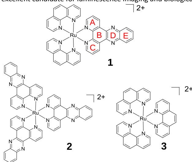
Fig. 1 The chemical structure of the 1 , 2 and 3 showing ring lettering codes used to describe the dppz ligand.
